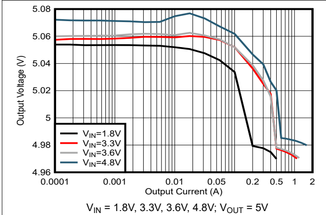
图 5-3. Load Regulation in Auto PFM with internal resistor divider (fixed 5.0V)
