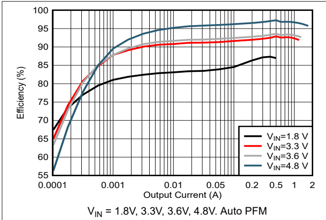
图 5-1. Efficiency vs Output Current V_{OUT} = 5V
