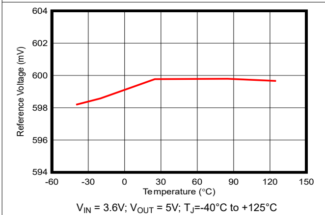
图 5-5. Reference Voltage vs Temperature
