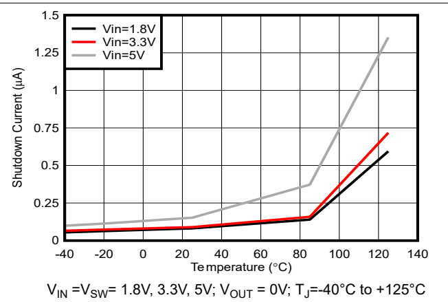
图 5-6. Shutdown Current vs Temperature
