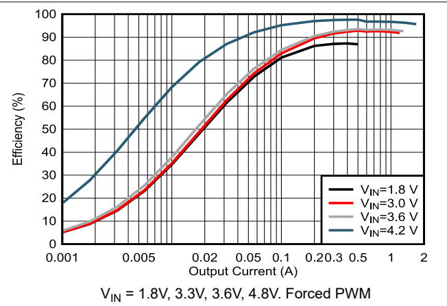
图 5-2. Efficiency vs Output Current V_{OUT} = 5V
