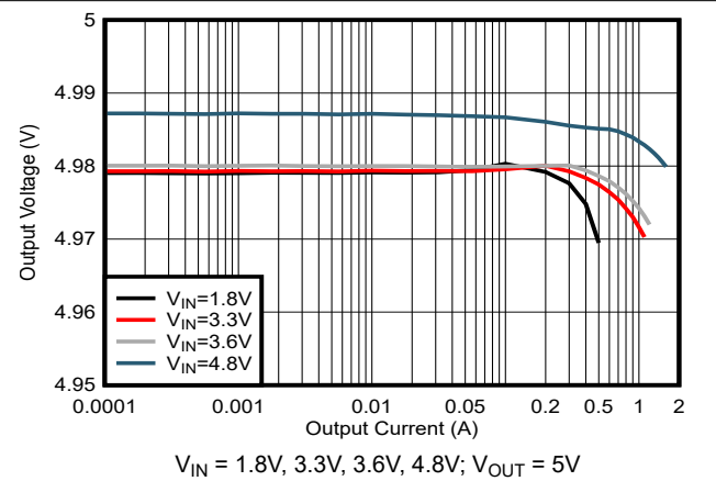
图 5-4. Load Regulation in Forced PWM with internal resistor divider (fixed 5.0V)
