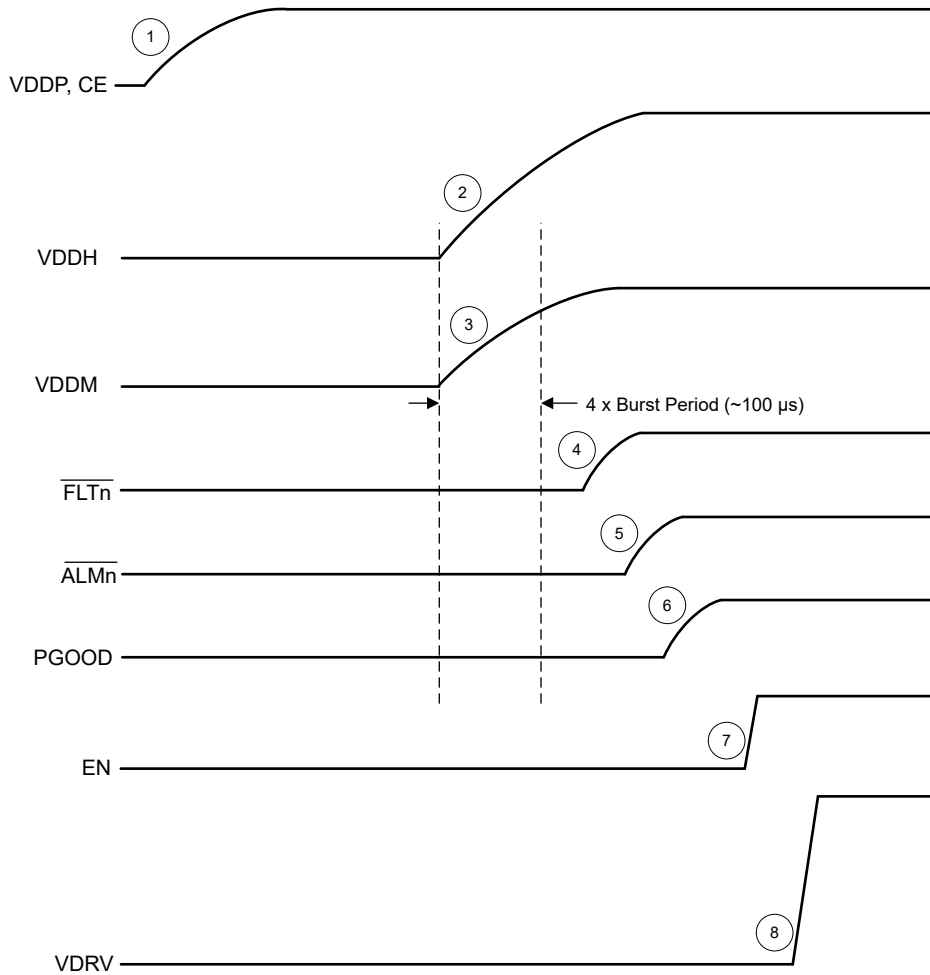
图 8-11. TPSI310x 典型启动 ( CE = VDDP , \overline{FLTn\_CMP} = 0 , \overline{ALMn\_CMP} = 0 )
