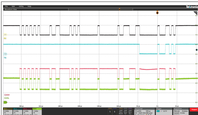
图 7-3. CAN Transceiver Operating
