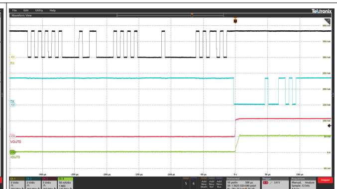
图 7-4. Output Control by FlexWire Interface
