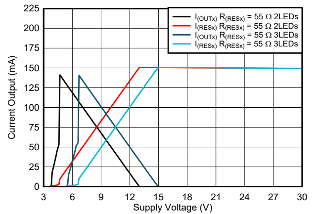
图 5-8. Output Current Distribution vs Supply Voltage
