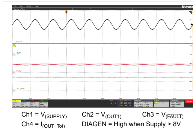
图 5-23. Superimposed Alternating Voltage 1kHz
