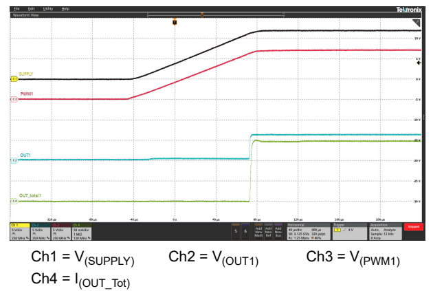
图 5-10. Power-Up Sequence
