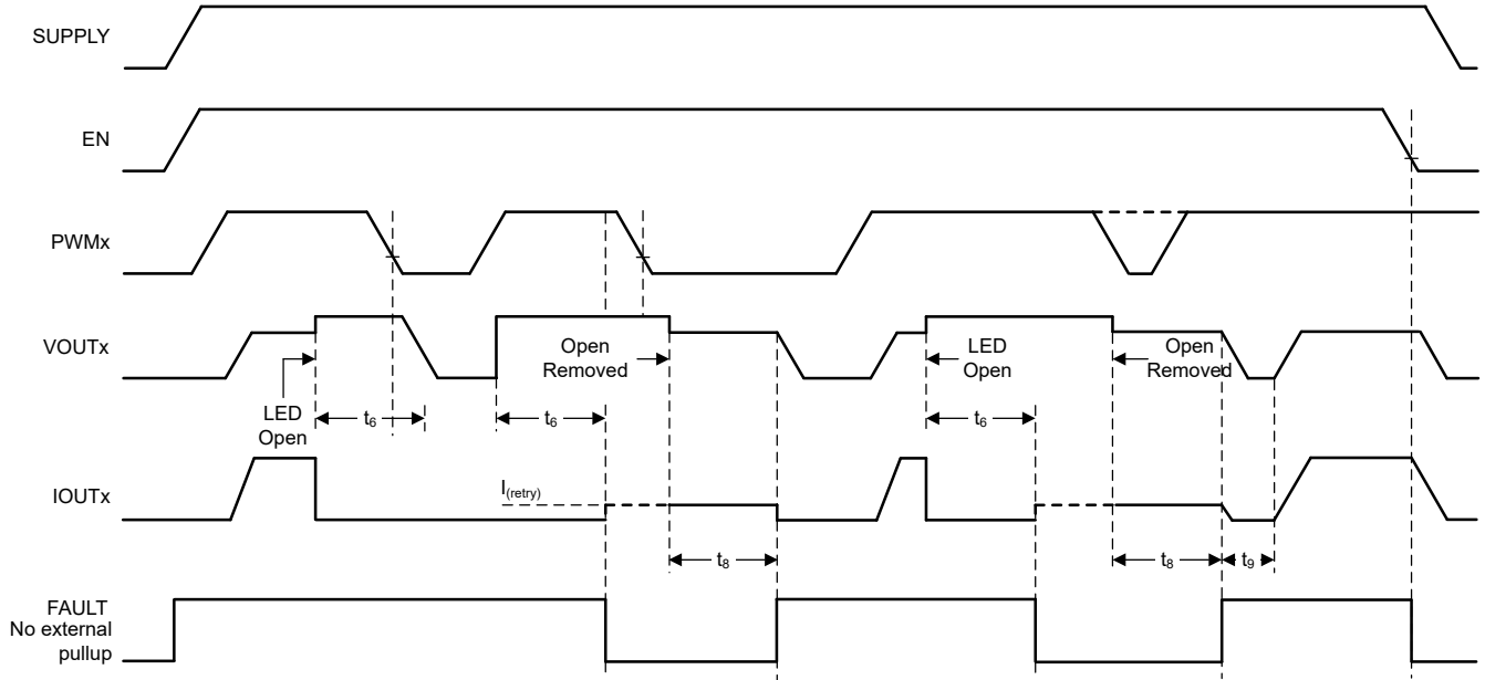
图 6-4. LED Open-Circuit Detection and Recovery Timing Diagram
