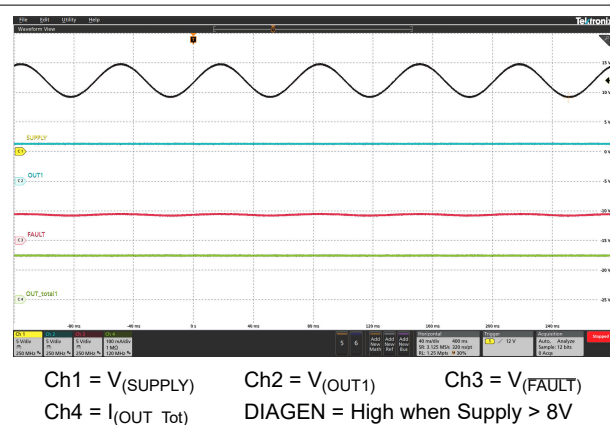
图 5-22. Superimposed Alternating Voltage 15Hz
