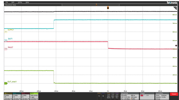
图 5-14. LED Open Protection
