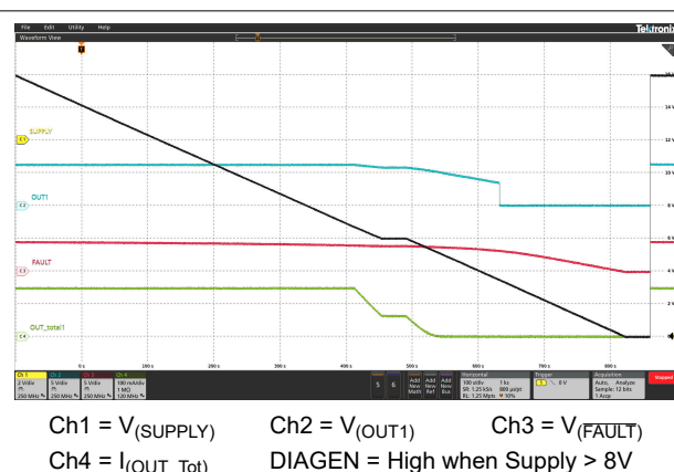
图 5-20. Slow Decrease and Quick Increase of Supply Voltage
