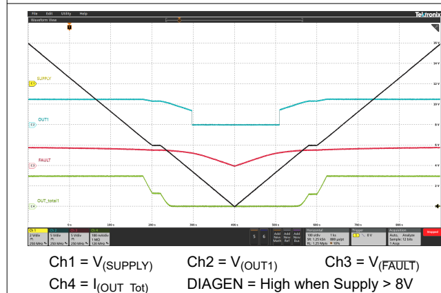
图 5-21. Slow Decrease and Slow Increase of Supply Voltage
