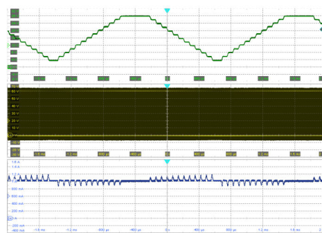
Ch1: SW voltage (10 V/div); Ch2: Output voltage (4 V/div); Ch4: LED current (200 mA/div); Time: 400 \mu s/div
