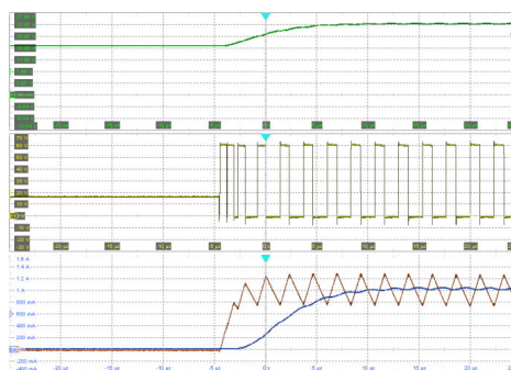
Ch1: SW voltage (10V/div); Ch2: Output voltage (4 V/div); Ch3: Inductor current (200 mA/div); Ch4: LED current (200 mA/div); Time: 5 \mu s/div
