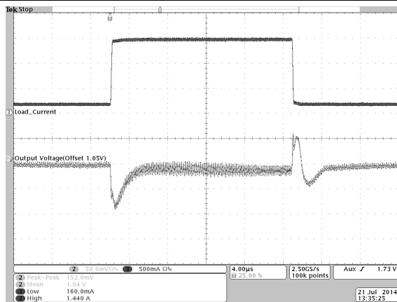
Figure 20. Load Transient Response for TPS8268105 ( V_{out} = 1.05V , I_{out} = 160mA to 1.44A to 160mA , V_{in} = 5V )
