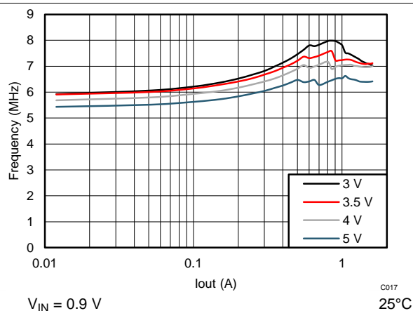
Figure 12. Switching Frequency vs Output Current
