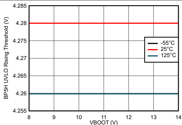
图 7-22. BP5H UVLO Rising Threshold vs BOOT Voltage
