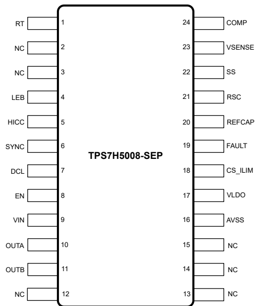
图 6-4. TPS7H5008-SEP PW Package 24-Pin TSSOP (Top View)
