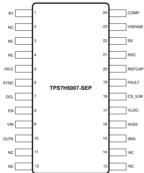
图 6-3. TPS7H5007-SEP PW Package 24-Pin TSSOP (Top View)
