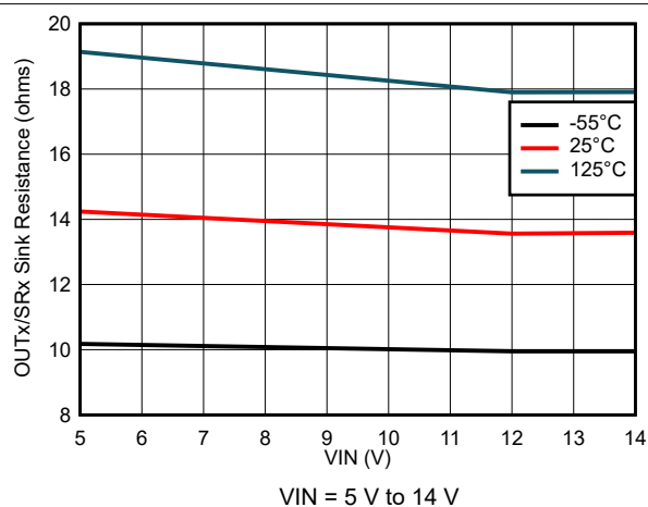
图 7-64. Output Sink Resistance Variation
