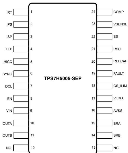
图 6-1. TPS7H5005-SEP PW Package 24-Pin TSSOP (Top View)
