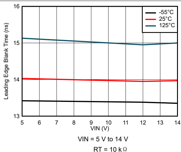
图 7-34. Leading Edge Blank Time Variation
