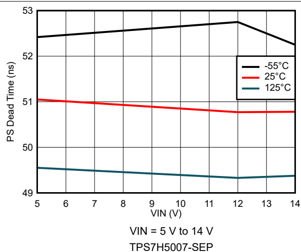
图 7-48. PS Dead Time Variation
