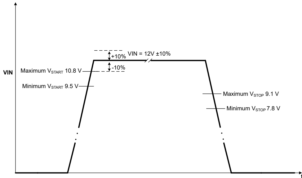
图 8-6. Start-Up and UVLO Values for Two-Resistor Configuration With VIN = 12 V
