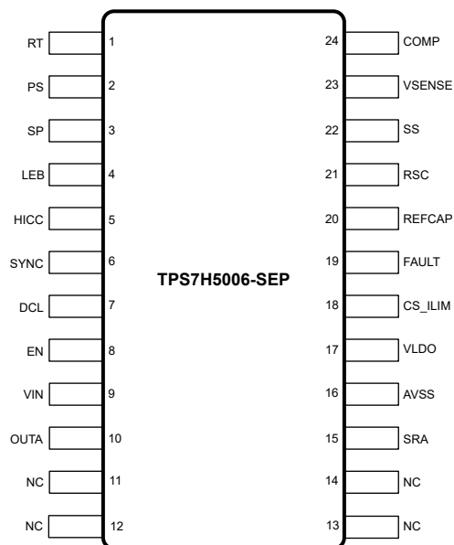
图 6-2. TPS7H5006-SEP PW Package 24-Pin TSSOP (Top View)
