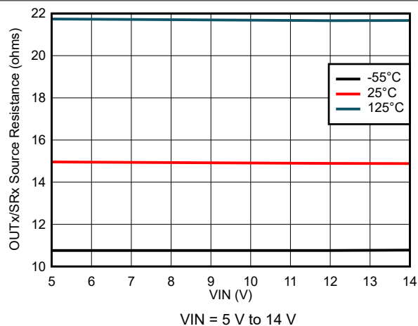
图 7-62. Output Source Resistance Variation
