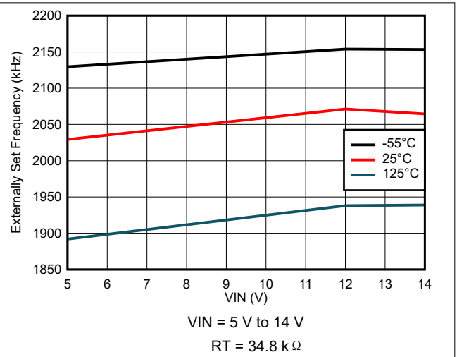
图 7-26. Externally Set Frequency Variation
