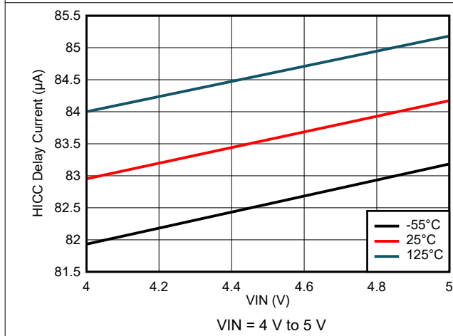
图 7-27. Hiccup Delay Current Variation
