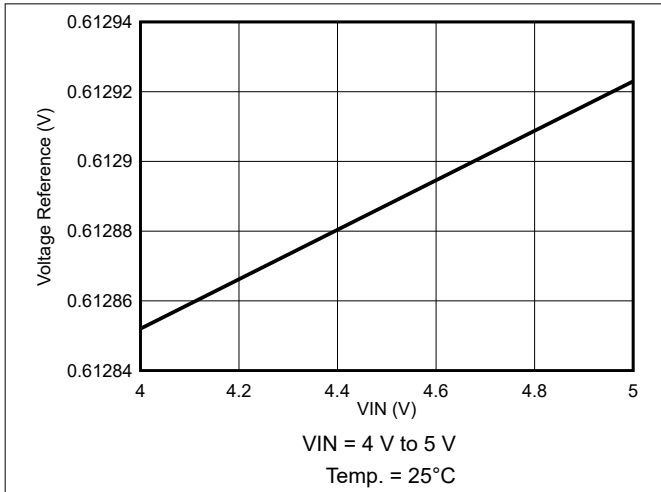
图 7-13. Voltage Reference Variation
