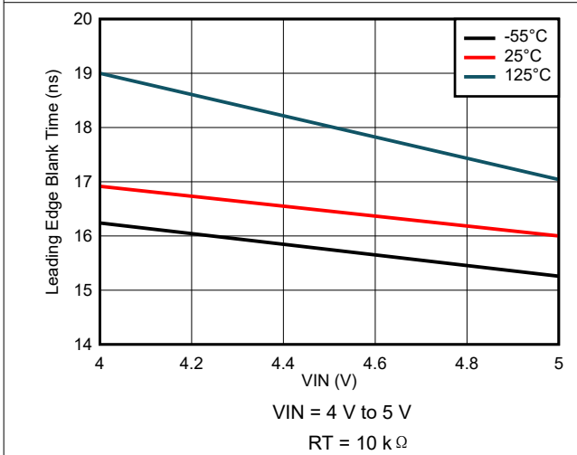
图 7-33. Leading Edge Blank Time Variation
