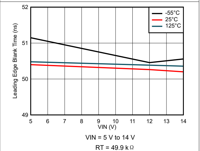
图 7-36. Leading Edge Blank Time Variation
