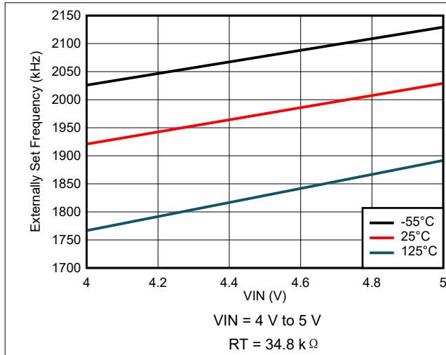
图 7-25. Externally Set Frequency Variation
