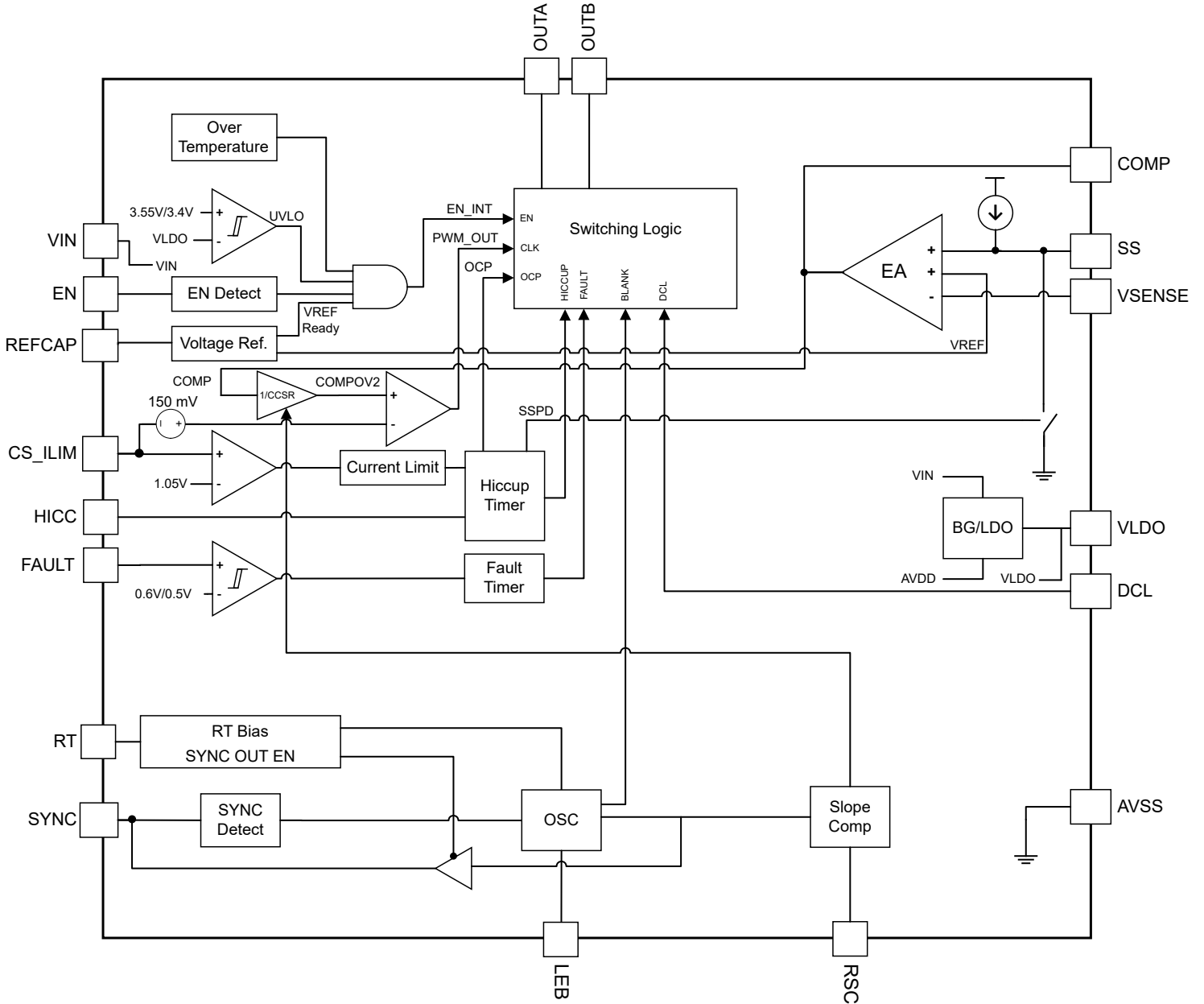
图 8-4. TPS7H5004-SP Functional Block Diagram
