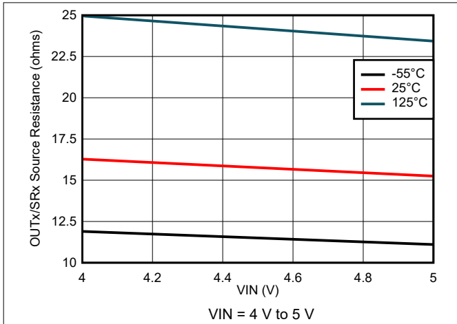
图 7-61. Output Source Resistance Variation
