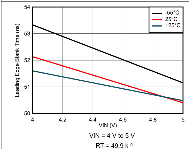
图 7-35. Leading Edge Blank Time Variation
