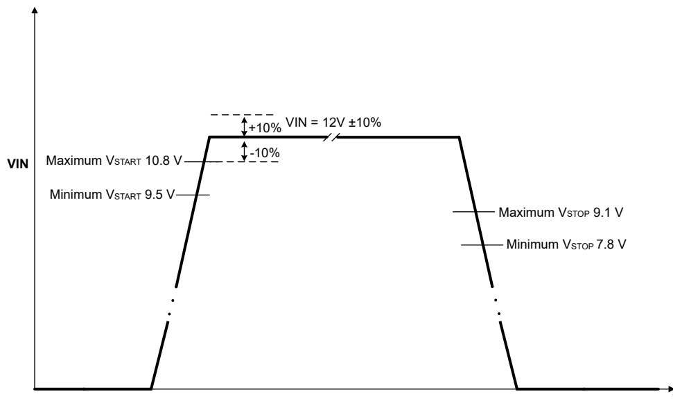
图 8-6. Start-Up and UVLO Values for Two-Resistor Configuration With V_{IN} = 12\text{ V}
