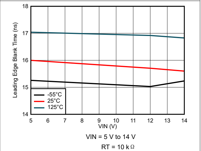
图 7-34. Leading Edge Blank Time Variation
