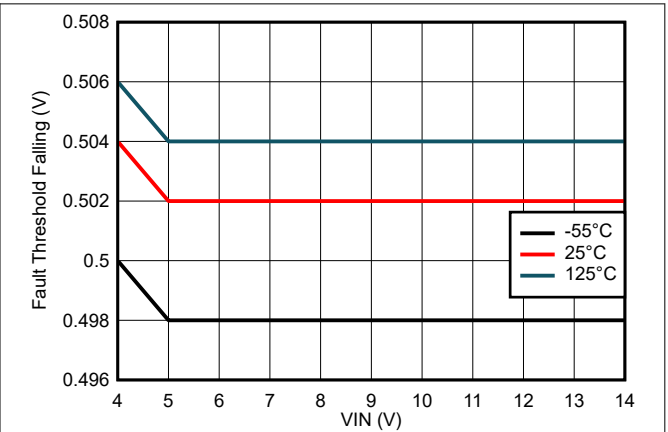
图 7-32. FAULT Threshold Falling Variation
