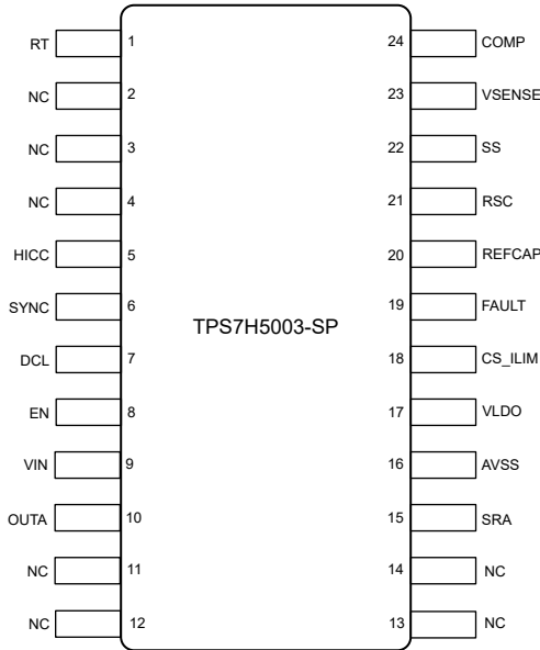
图 6-7. TPS7H5003-SP PW Package 24-Pin TSSOP (Top View)
