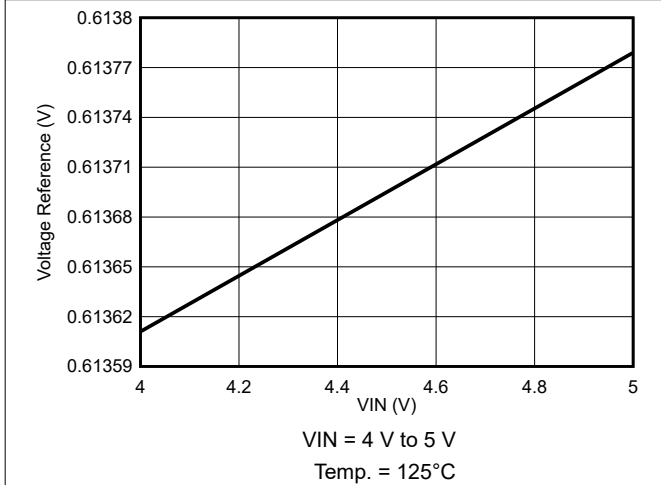
图 7-15. Voltage Reference Variation
