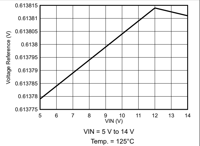
图 7-16. Voltage Reference Variation
