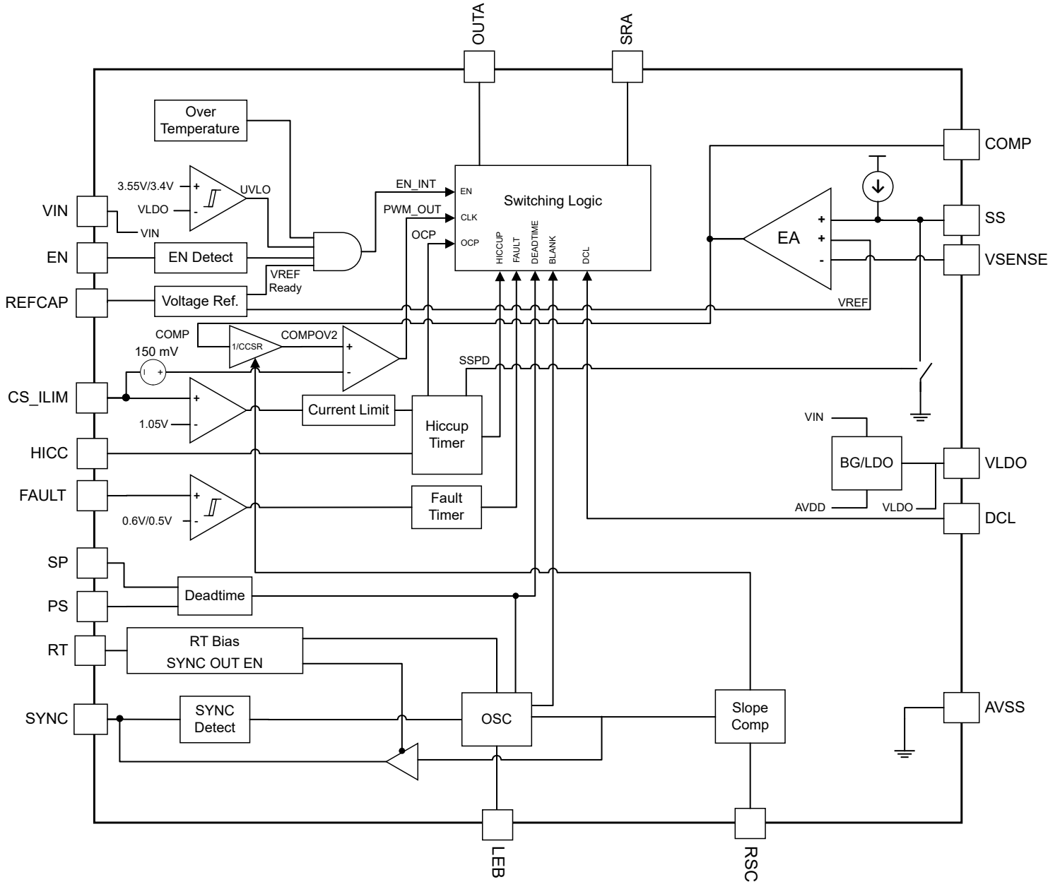
图 8-2. TPS7H5002-SP Functional Block Diagram
