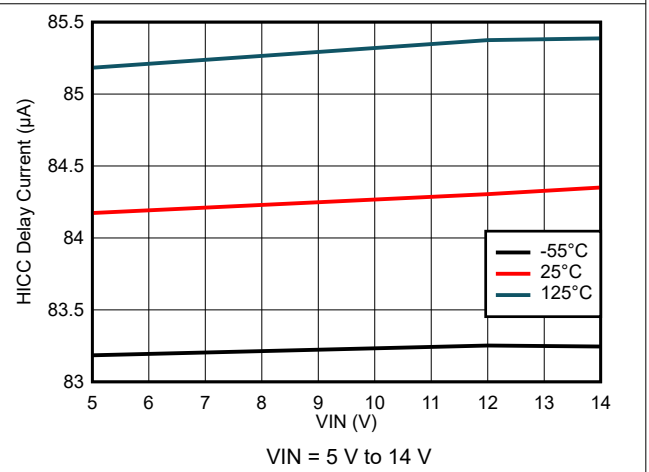
图 7-28. Hiccup Delay Current Variation
