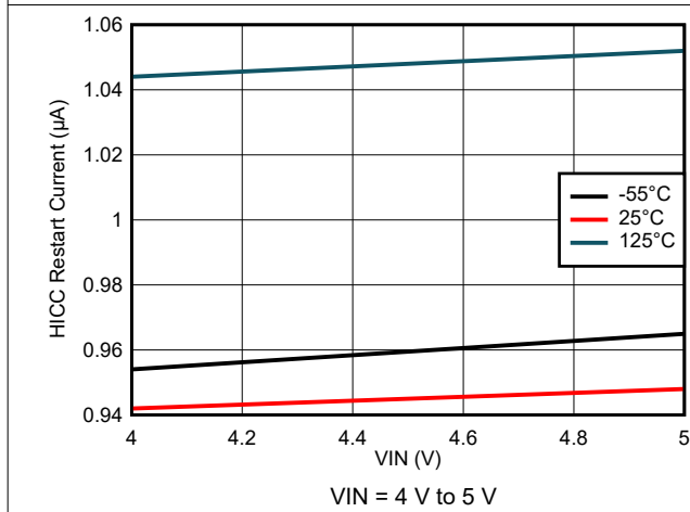
图 7-29. Hiccup Restart Current Variation
