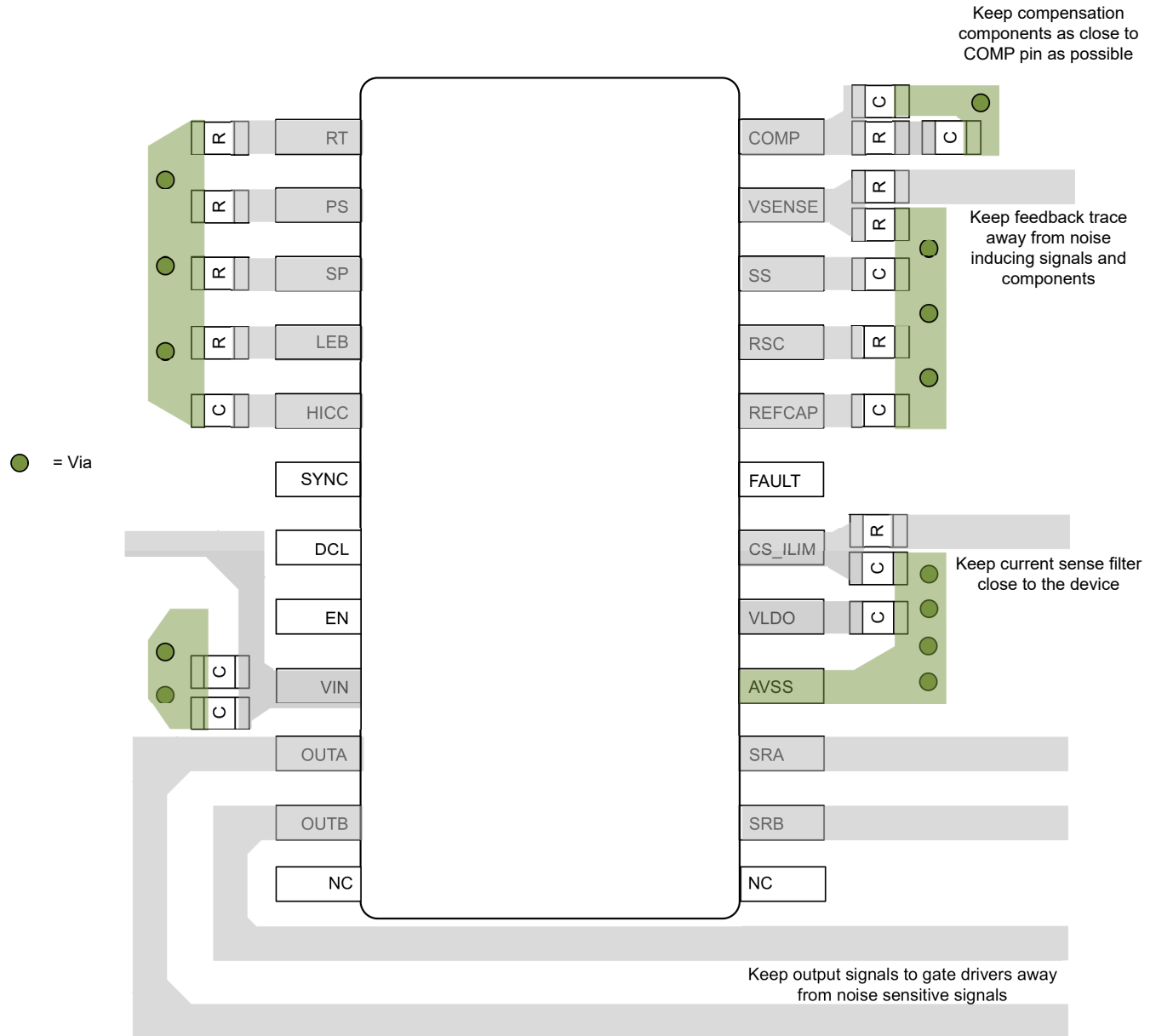
图 9-5. PCB Layout Example for TSSOP Package
