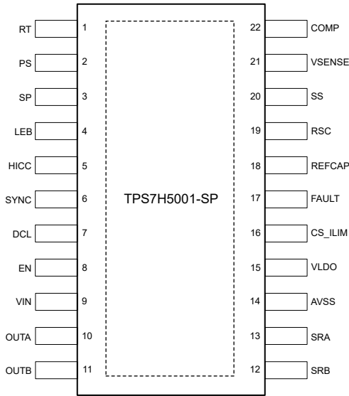
图 6-1. TPS7H5001-SP HFT Package 22-Pin CFP With Thermal Pad (Top View)
