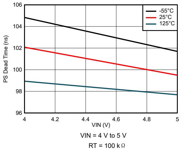
图 7-45. PS Dead Time Variation
