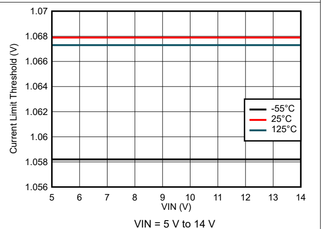
图 7-18. Current Limit Threshold Variation
