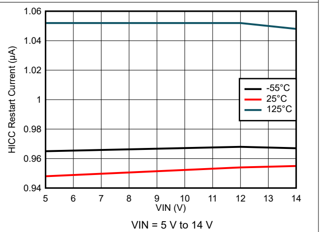
图 7-30. Hiccup Restart Current Variation
