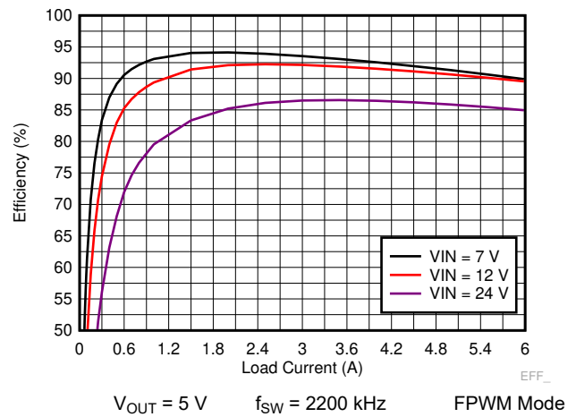
图 8-8. TPS7H4010-SEP Efficiency
