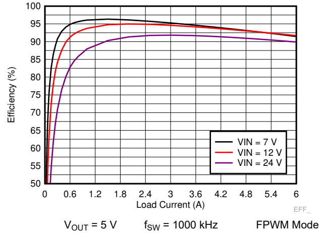
图 8-6. TPS7H4010-SEP Efficiency
