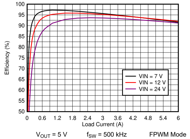
图 8-4. TPS7H4010-SEP Efficiency
