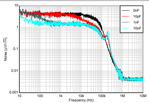
V_{IN} = 4.3\text{V} , V_{OUT} = 3.3\text{V} , C_{OUT} = 2.2\mu\text{F} , I_{OUT} = 150\text{mA}
