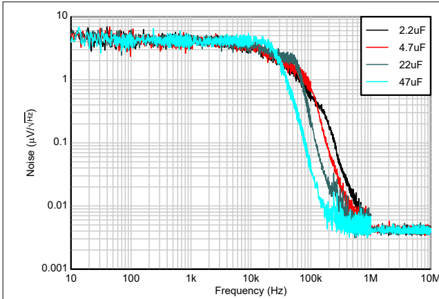
V_{IN} = 4.3\text{V} , V_{OUT} = 3.3\text{V} , I_{OUT} = 150\text{mA}
