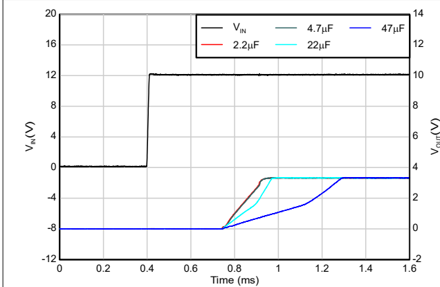
V_{IN} = 12\text{V} , V_{OUT} = 3.3\text{V} , I_{OUT} = 1\text{mA}
