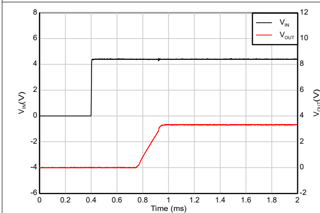
V_{IN} = 4.3\text{V} , V_{OUT} = 3.3\text{V} , I_{OUT} = 1\text{mA}
