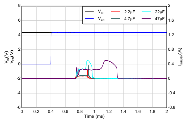
V_{IN} = 4.3\text{V} , V_{OUT} = 3.3\text{V} , I_{OUT} = 0\text{mA}
