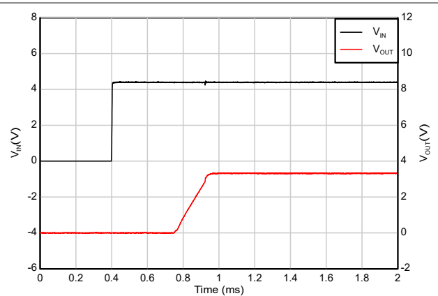
V_{IN} = 4.3\text{V} , V_{OUT} = 3.3\text{V} , I_{OUT} = 10\text{mA}
