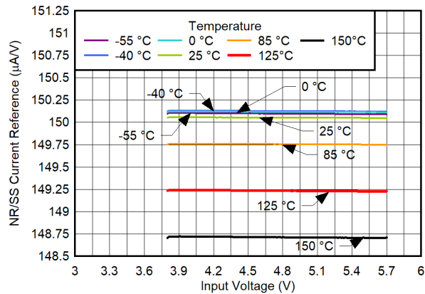
图 8-11. I_{NR/SS} Reference vs Input Voltage and Temperature for V_{OUT} = 3.3\text{ V}
