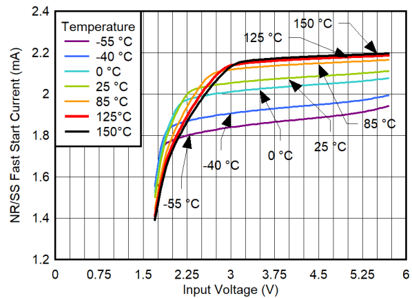
图 8-12. I_{FAST\_SS} Reference vs Input Voltage and Temperature for V_{OUT} = 3.3\text{ V}
