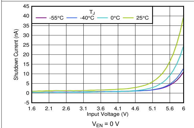
图 5-41. Shutdown Current vs V_{IN}
