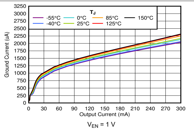
图 5-38. I_{GND} vs I_{OUT}
