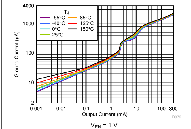
图 5-39. I_{GND} vs I_{OUT}
