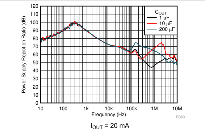
图 5-64. PSRR vs Frequency and C_{OUT}
