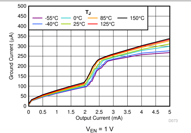
图 5-40. I_{GND} vs I_{OUT}
