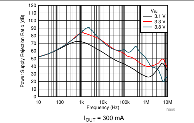
图 5-62. PSRR vs Frequency and V_{IN}
