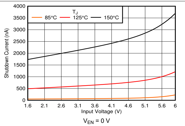
图 5-42. Shutdown Current vs V_{IN}
