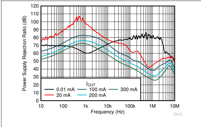
图 5-63. PSRR vs Frequency and I_{OUT}
