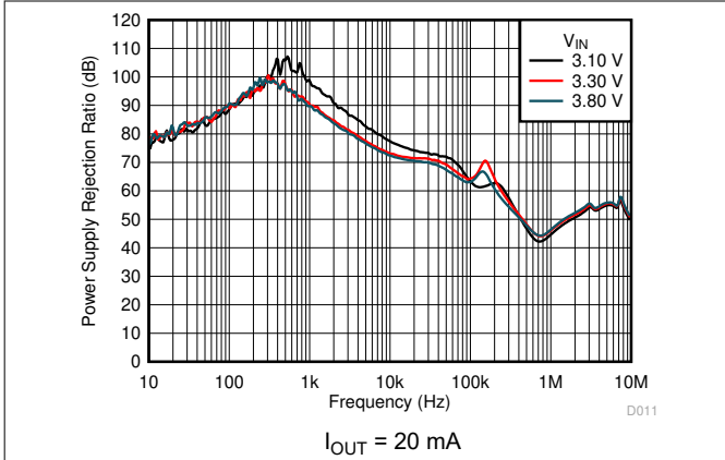
图 5-61. PSRR vs V_{IN} vs Frequency and V_{IN}
