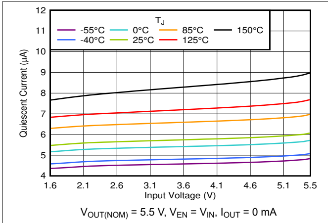
图 5-37. I_{GND} vs V_{IN} in the Dropout Region
