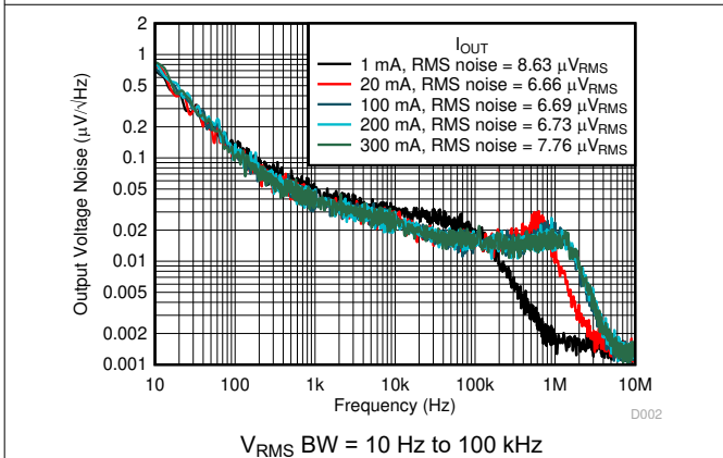
图 5-65. Noise vs Frequency and I_{OUT}
