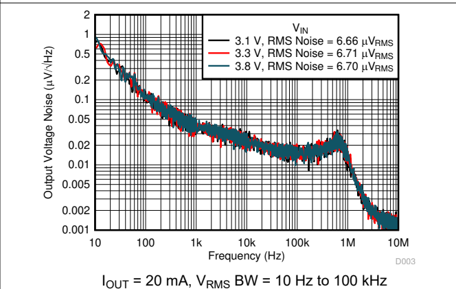
图 5-66. Noise vs Frequency and V_{IN}
