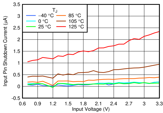
V_{OUT} = 1.0\text{ V} , V_{EN} < 0.4\text{ V} 图 6-13. I_{SHDN} vs V_{IN} and Temperature
