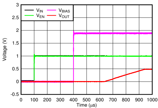
V_{OUT} = 0.5\text{ V} 图 6-17. Startup With V_{BIAS} Powering Up After V_{IN} and V_{EN}
