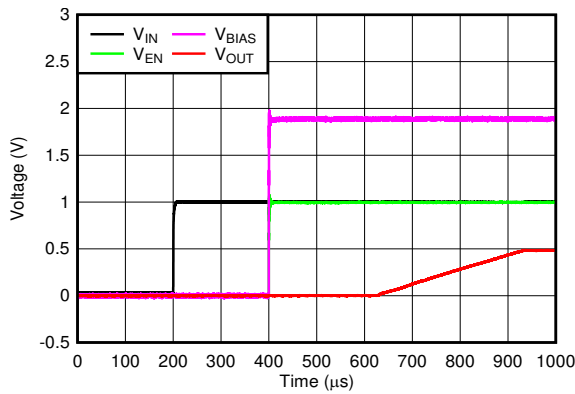
V_{OUT} = 0.5\text{ V} 图 6-15. Startup With V_{EN} and V_{BIAS} Powering Up Simultaneously
