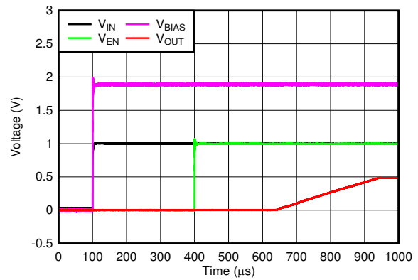
V_{OUT} = 0.5\text{ V} 图 6-16. Startup With Separated V_{EN}
