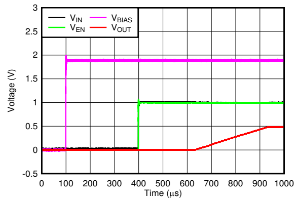
V_{OUT} = 0.5\text{ V} 图 6-14. Startup With V_{EN} = V_{IN}
