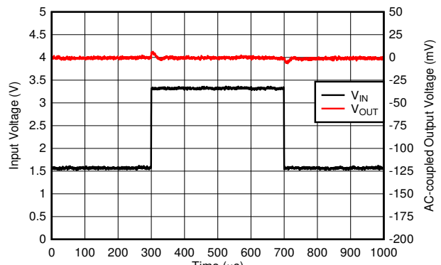
V_{OUT} = 1.0\text{ V} , I_{OUT} = 1\text{ mA} 图 6-18. V_{IN} Transient
