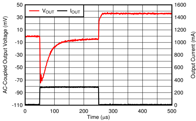
V_{\text{OUT}} = 3.3\text{ V} , I_{\text{OUT}} = 0\text{ mA to } 300\text{ mA} , I_{\text{OUT}}\text{ slew rate} = 1\text{ A}/\mu\text{s} , T_J = 150^\circ\text{C}
