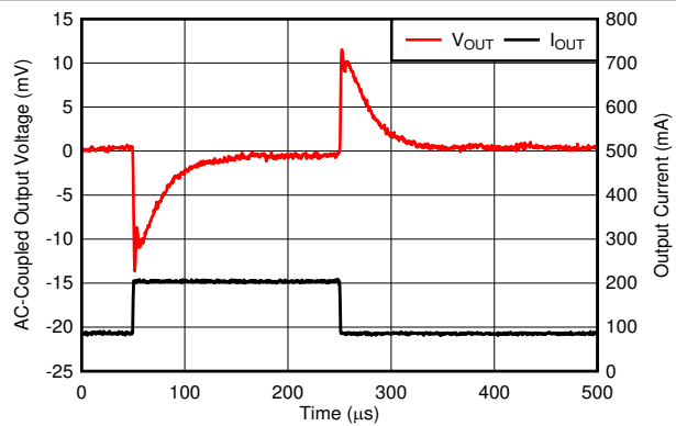
V_{\text{OUT}} = 3.3\text{ V} , I_{\text{OUT}} = 90\text{ mA to } 200\text{ mA} , I_{\text{OUT}}\text{ slew rate} = 1\text{ A}/\mu\text{s} , T_J = 150^\circ\text{C}
