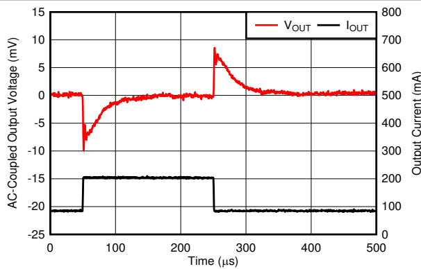
V_{\text{OUT}} = 3.3\text{ V} , I_{\text{OUT}} = 90\text{ mA to } 200\text{ mA} , I_{\text{OUT}}\text{ slew rate} = 1\text{ A}/\mu\text{s} , T_J = -40^\circ\text{C}
