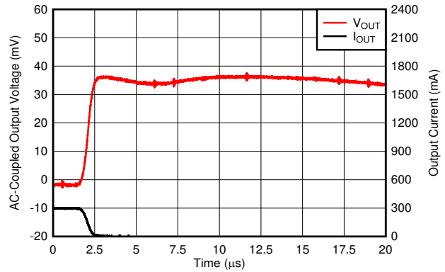
图 6-20. I_{\text{OUT}} Transient From 300 mA to 1 mA
