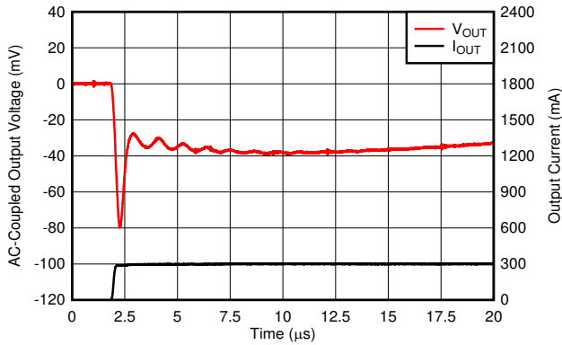
图 6-19. I_{\text{OUT}} Transient From 1 mA to 300 mA
