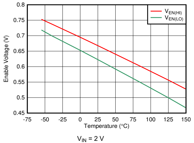
图 6-12. V_{EN(HI)} and V_{EV(LO)} Threshold vs Temperature
