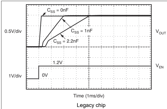
图 5-38. Turn-On Response
