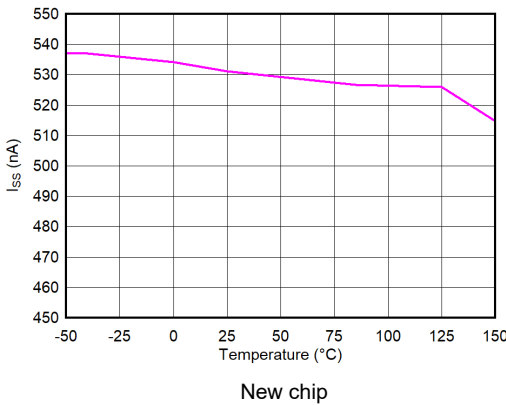
图 5-27. Soft-Start Charging Current (I SS ) vs Temperature (T J )
