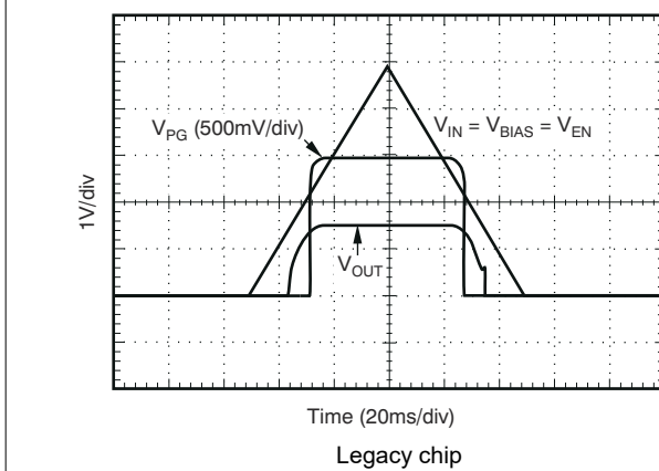
图 5-40. Power-Up, Power-Down
