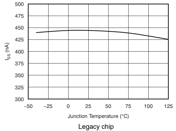
图 5-26. Soft-Start Charging Current (I SS ) vs Temperature (T J )
