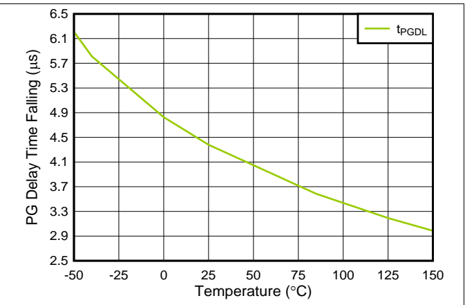
图 20. t_{PGDL} vs Temperature
