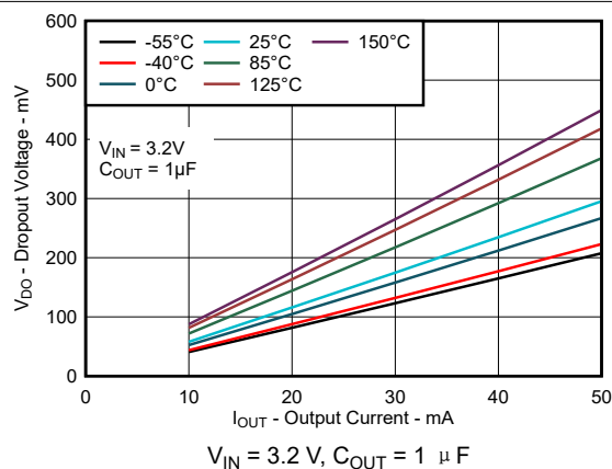
图 6-10. Dropout Voltage vs Output Current for New Chip
