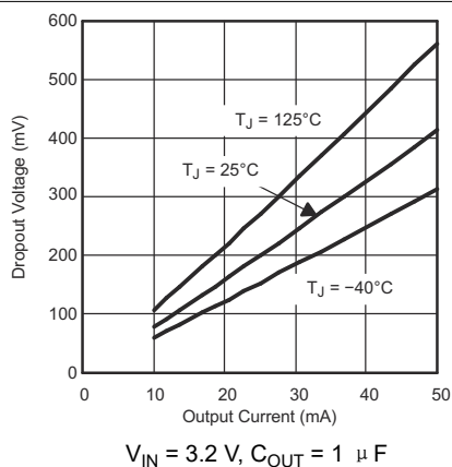
图 6-9. Dropout Voltage vs Output Current for Legacy Chip
