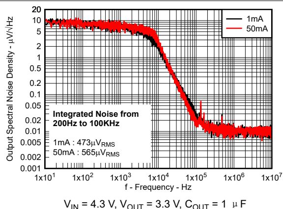
图 6-8. Output Spectral Noise Density vs Frequency for New Chip
