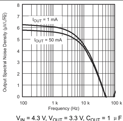
图 6-7. Output Spectral Noise Density vs Frequency for Legacy Chip
