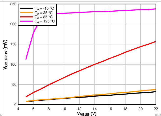
图 4. V_{OC\_PP1HV} , PPHV Open Circuit Voltage versus VBUS
