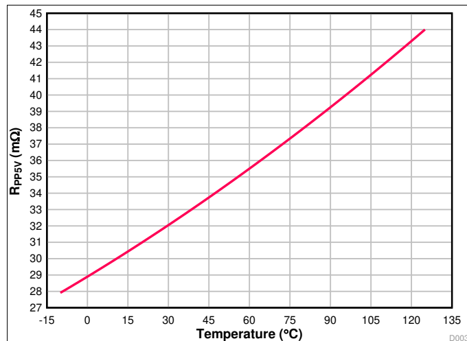
图 1. R_{PP5V} versus Temperature
