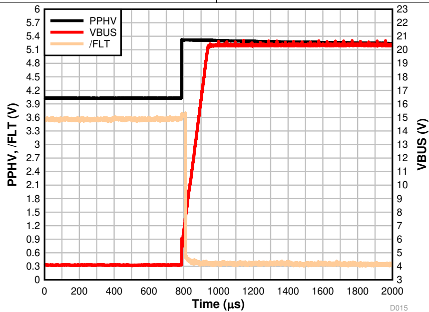
图 9. VBUS OVP Response with 6-V Threshold
