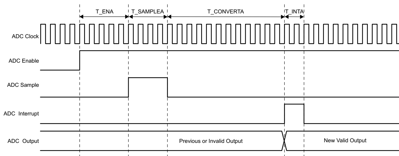
图 7-2. ADC Enable and Conversion Timing
