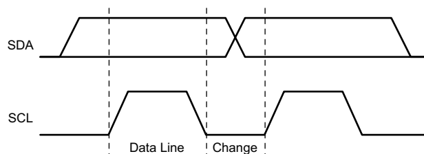
图 8-22. I 2 C Bit Transfer
