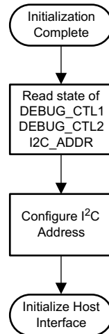
图 8-17. I 2 C Address Configuration
