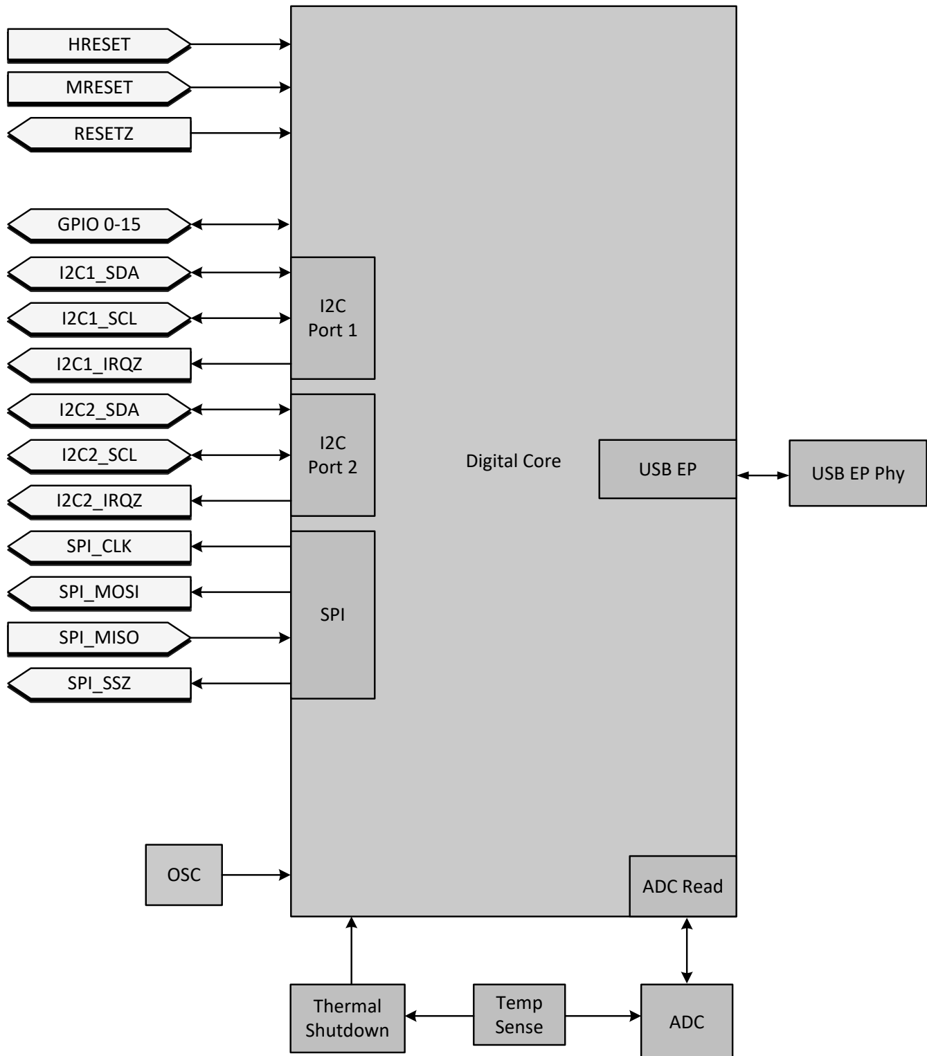
图 8-8. Digital Core Block Diagram
