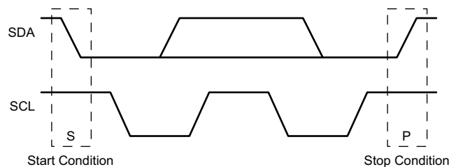
图 8-21. I 2 C Definition of Start and Stop Conditions
