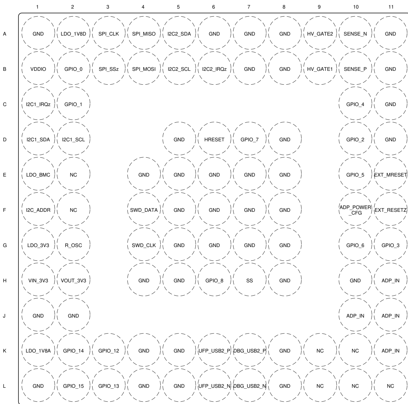
图 5-1. ZBH Package 96-Pin NFBGA Top View
