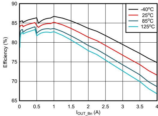
图 9-10. BUCK Efficiency at different T_A , Auto Mode
