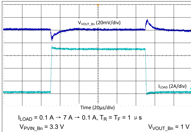
图 9-40. Buck Load Step Transient - 4-Phase, 2.2 MHz, Forced-PWM Mode
