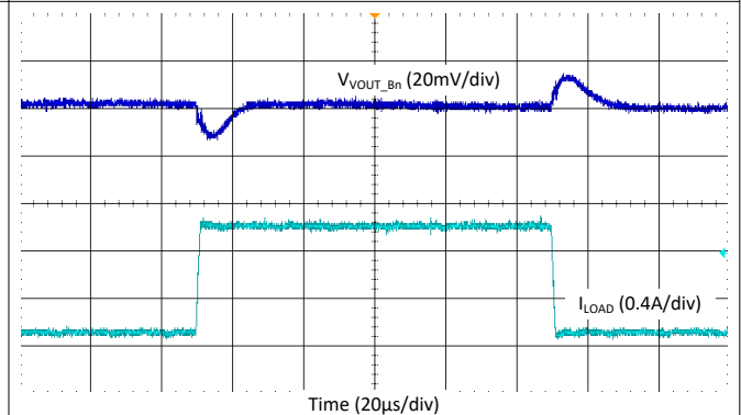
图 9-55. Buck Load Step Transient - Buck5, 4.4 MHz, Auto Mode
