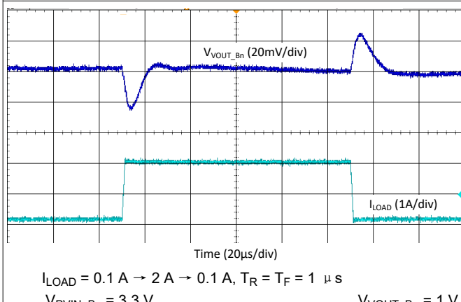
图 9-50. Buck Load Step Transient - Buck4, 2.2 MHz, Auto Mode
