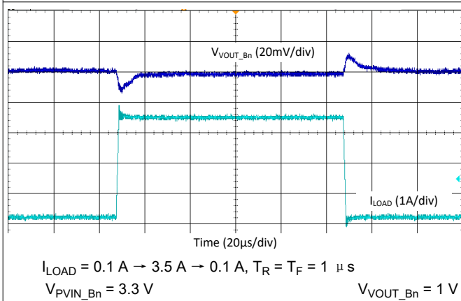
图 9-48. Buck Load Step Transient - 2-Phase, 2.2 MHz, Forced-PWM Mode
