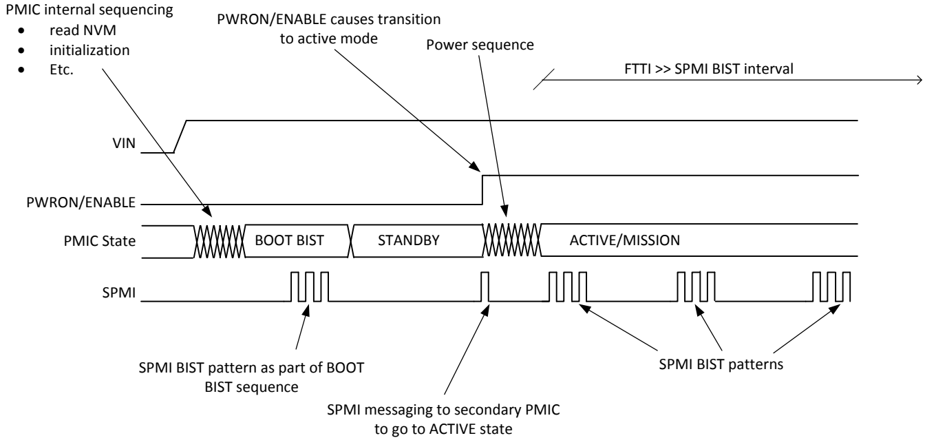
图 8-50. SPMI-BIST Operation
