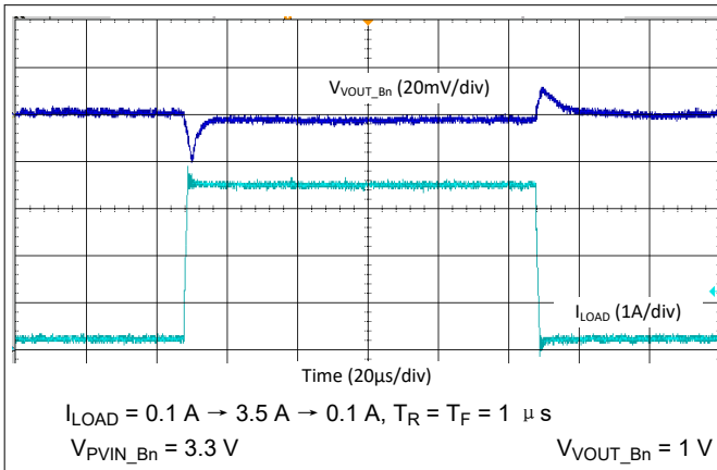
图 9-46. Buck Load Step Transient - 2-Phase, 2.2 MHz, Auto Mode
