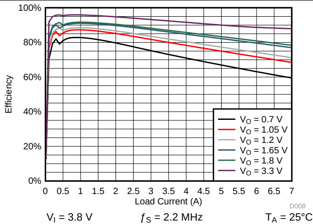
图 4-10. SMPS Efficiency for SMPS12 in Dual-Phase PWM Mode
