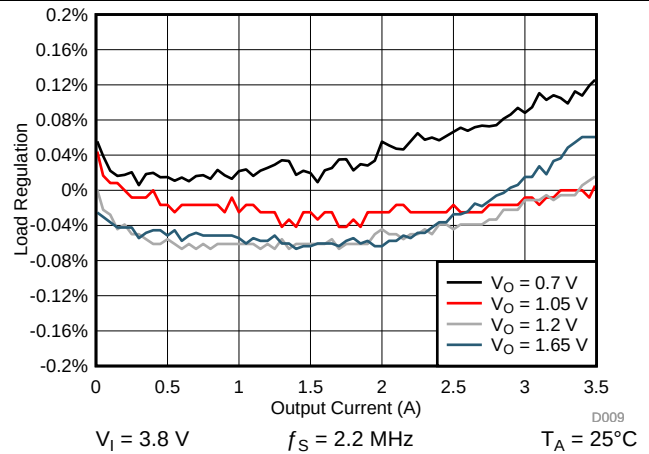
图 4-11. SMPS Load Regulation for SMPS1 and SMPS2 Single-Phase PWM Mode
