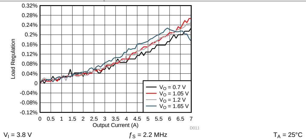
图 4-14. SMPS Load Regulation for SMPS12 in Dual-Phase PWM Mode
