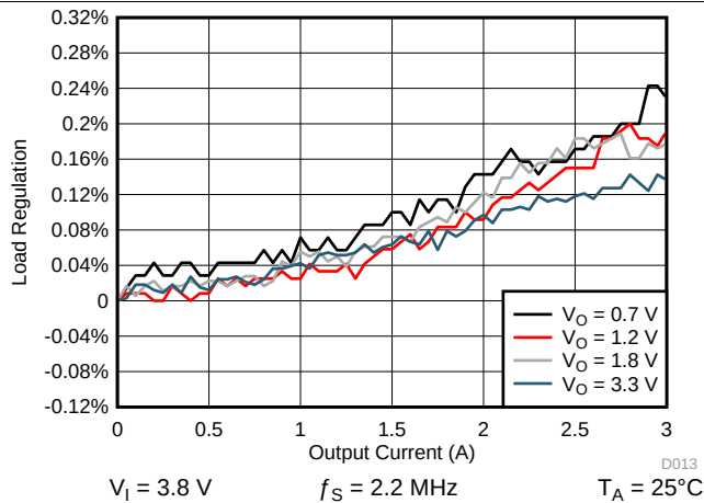
图 4-12. SMPS Load Regulation for SMPS3, PWM Mode
