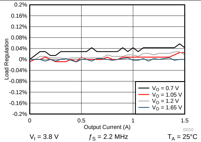
图 4-13. SMPS Load Regulation for SMPS4 in PWM Mode
