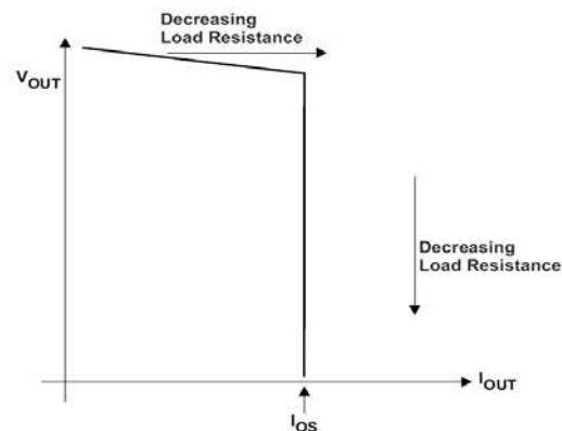
Figure 3. Output Voltage vs Current Limit Threshold
