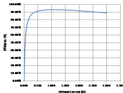
Figure 15. Buck Efficiency
