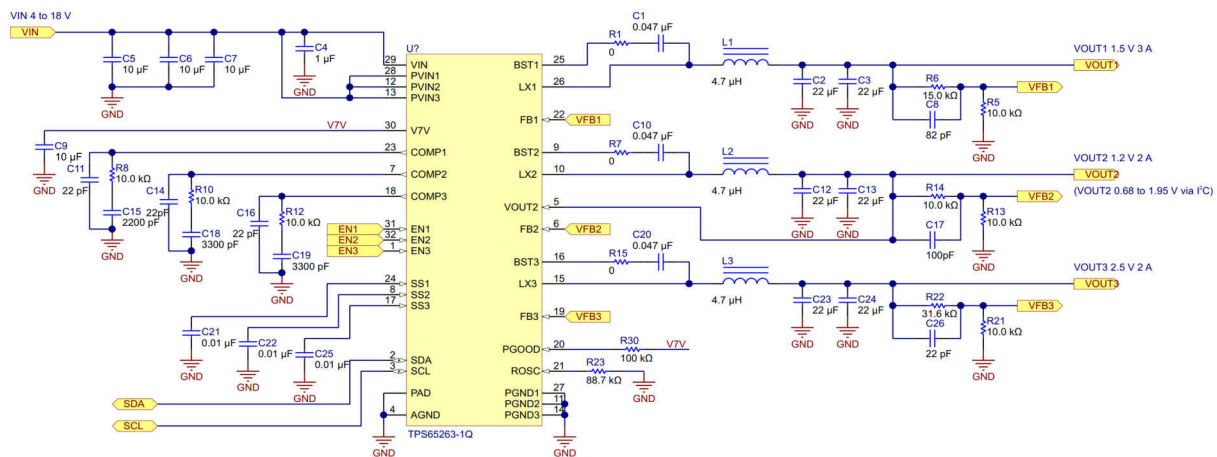
图 8-1. Typical Application Schematic
