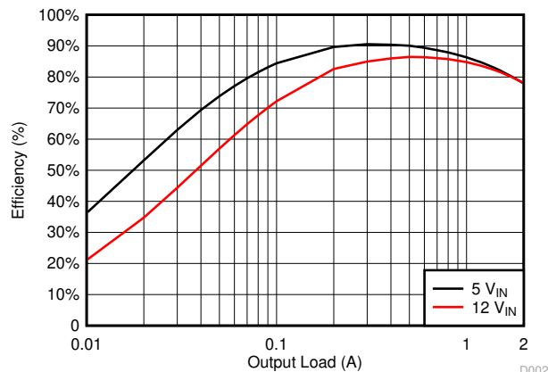
图 6-1. BUCK1 Efficiency
