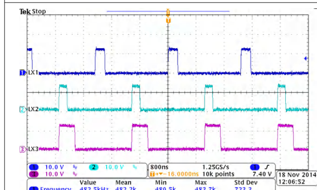
图 8-21. 180° Out-of-Phase
