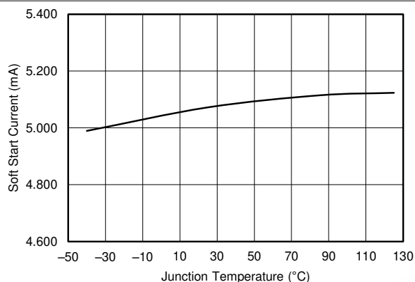
图 7-17. SS Pin Charge Current vs Temperature
