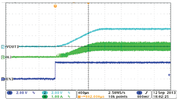
图 8-8. PSM Mode Buck3, Soft-Start with Full Load
