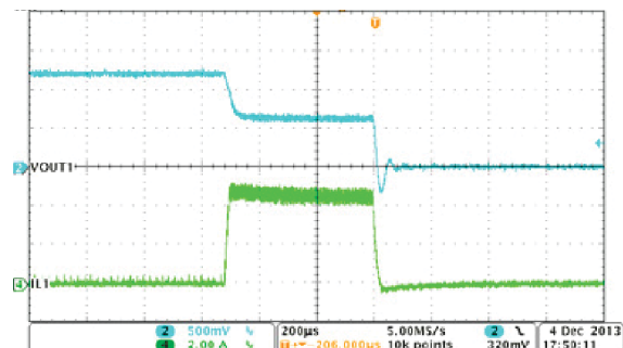
图 8-21. Buck1, Overcurrent Protection
