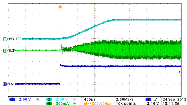
图 8-31. PWM Mode, Buck3, Soft-Start with No Load
