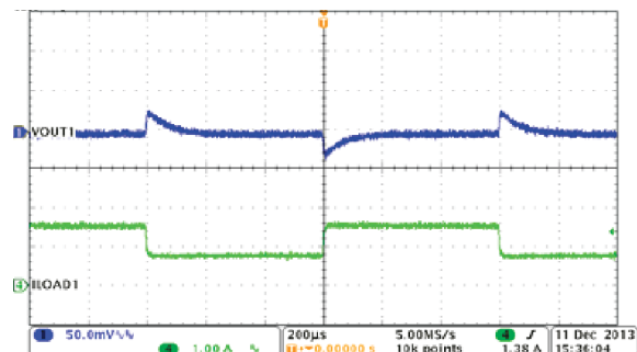
图 8-15. Buck1, Load Transient, 0.75 to 1.5 A SR = 0.25 A/µs
