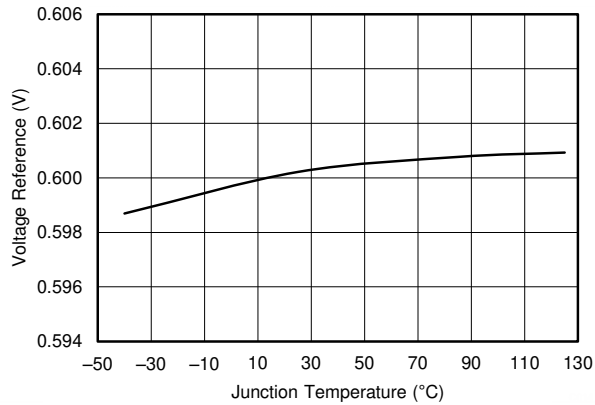
图 6-13. Voltage Reference vs Temperature
