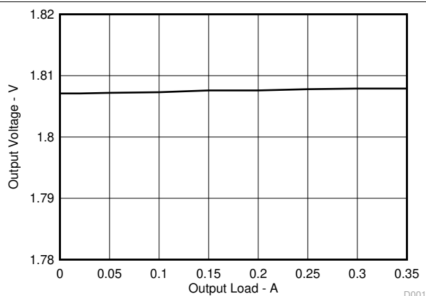
图 6-9. LDO1, Load Regulation, V_{IN} = 3.3\text{ V}
