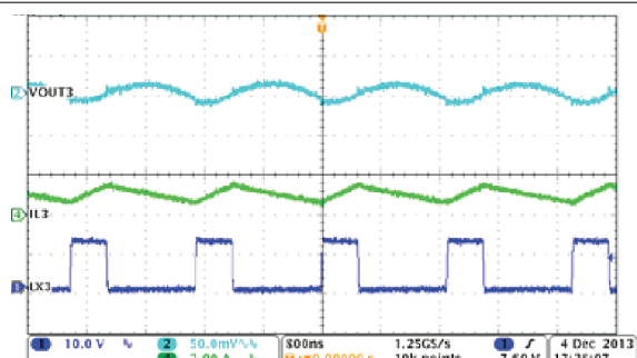
图 8-14. Buck3, Steady State Operation with Full Load
