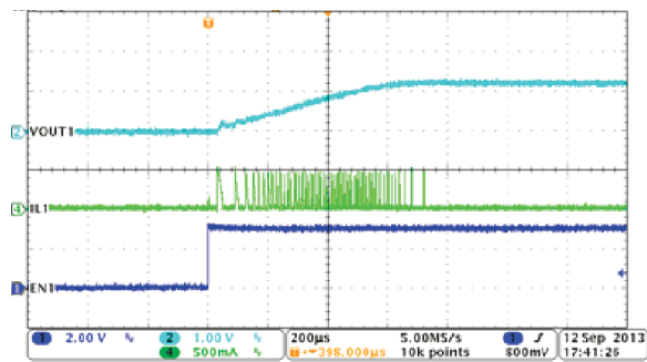
图 8-3. PSM Mode Buck1, Soft-Start with No Load
