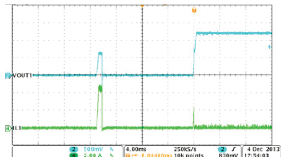
图 8-22. Buck1, Hiccup and Recovery
