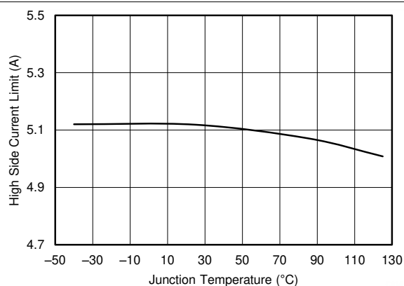
图 6-21. Buck1 High-Side Current Limit vs Temperature
