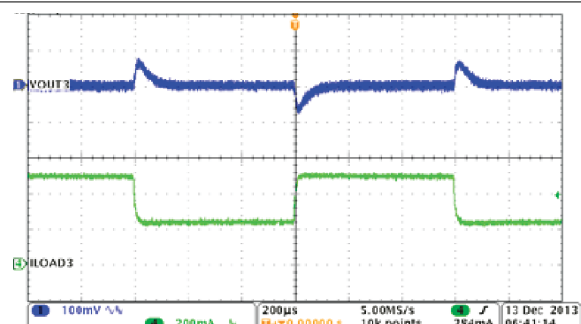
图 8-19. Buck3, Load Transient, 0.25 to 0.5 A SR = 0.25 A/µs
