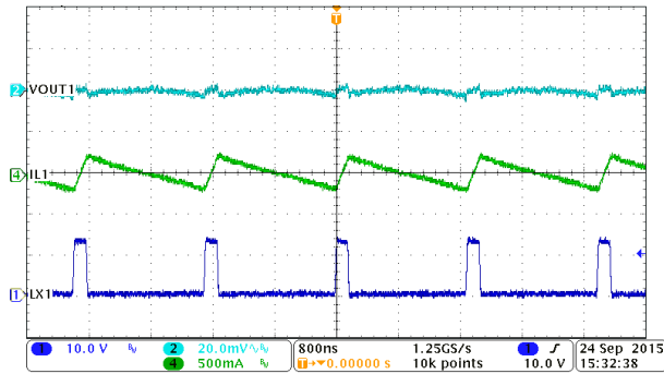
图 8-33. PWM Mode, Buck1, Steady State Operation with No Load
