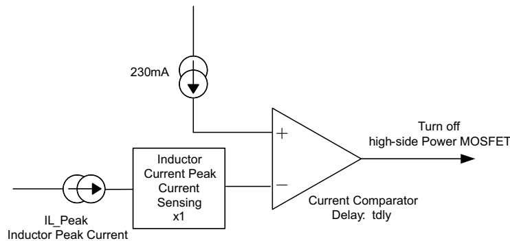
图 7-5. PSM Current Comparator
