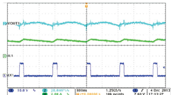
图 8-10. Buck1, Steady State Operation with Full Load
