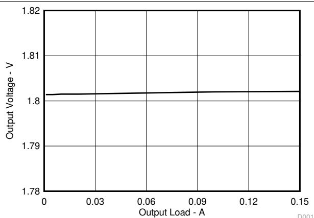
图 6-10. LDO2, Load Regulation, V_{IN} = 3.3\text{ V}
