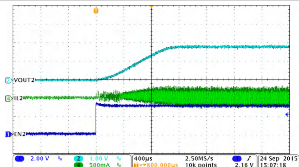
图 8-29. PWM Mode, Buck2, Soft-Start with No Load
