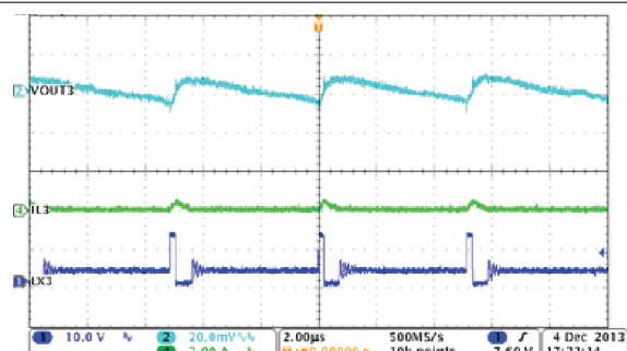
图 8-13. PSM Mode Buck3, Steady State Operation with Light Load
