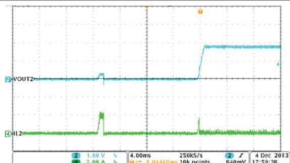
图 8-24. Buck2, Hiccup and Recovery
