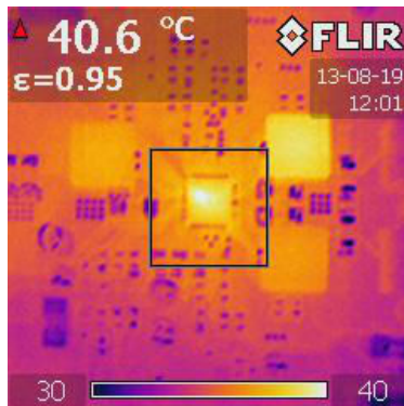
图 8-33. PWM Mode, Buck1, Steady State Operation with No Load
