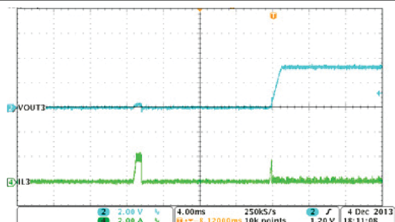
图 8-26. Buck3, Hiccup and Recovery
