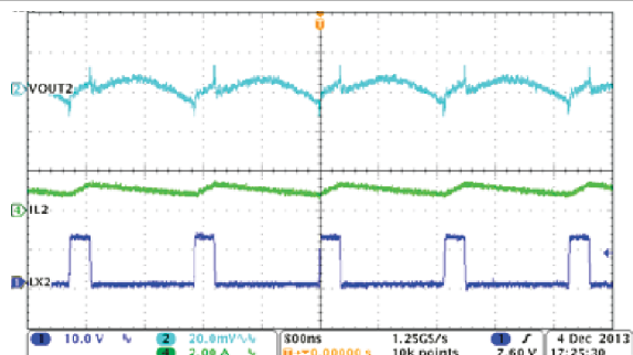
图 8-12. Buck2, Steady State Operation with Full Load
