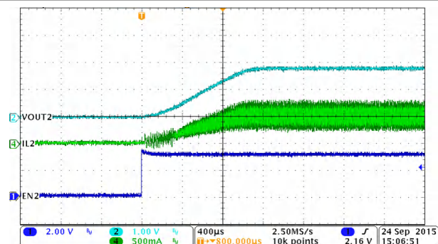
图 8-30. PWM Mode, Buck2, Soft-Start with Full Load
