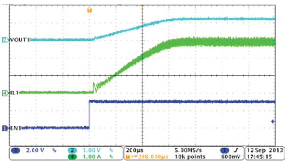
图 8-4. PSM Mode Buck1, Soft-Start With Full Load
