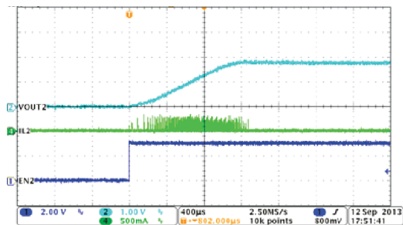
图 8-5. PSM Mode Buck2, Soft-Start with No Load
