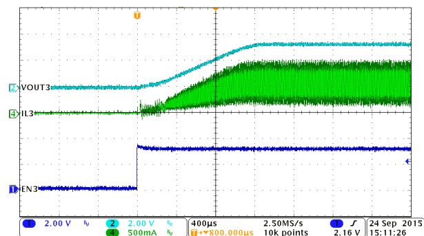
图 8-32. PWM Mode, Buck3, Soft-Start with Full Load
