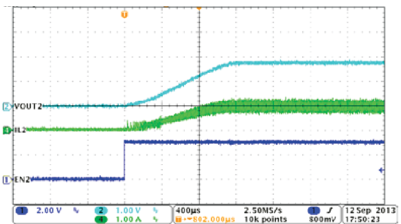
图 8-6. PSM Mode Buck2, Soft-Start with Full Load
