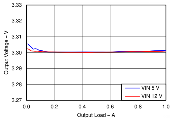
图 6-5. Buck3, PSM Mode Load Regulation
