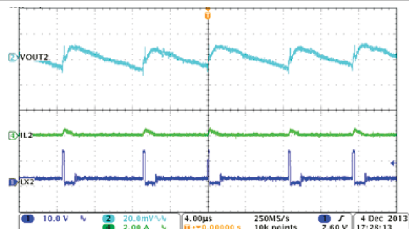
图 8-11. PSM Mode Buck2, Steady State Operation With Light Load
