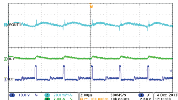
图 8-9. PSM Mode Buck1, Steady State Operation with Light Load
