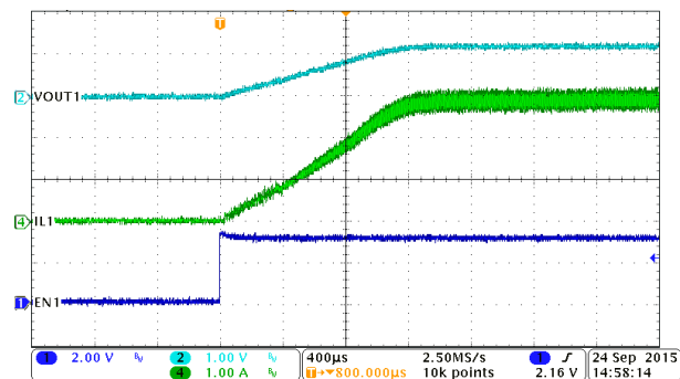
图 8-28. PWM Mode, Buck1, Soft-Start with Full Load
