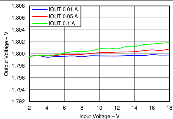
图 6-12. LDO2, Line Regulation
