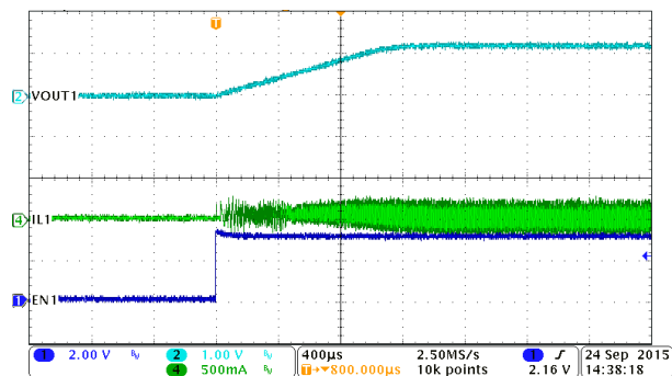
图 8-27. PWM Mode, Buck1, Soft-Start with No Load
