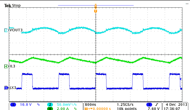
图 9-13. Buck3, Steady State Operation at Full Load
