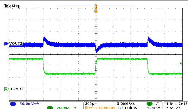
图 9-16. Buck2, Load Transient, 0.25 to 0.5 A SR = 0.25 A/μs
