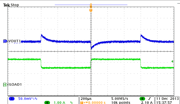
图 9-15. Buck1, Load Transient, 1.5 to 2.25 A SR = 0.25 A/μs
