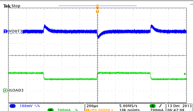
图 9-19. Buck3, Load Transient, 0.5 to 0.75 A SR = 0.25 A/μs
