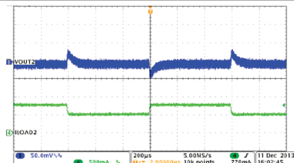
图 8-18. Buck2, Load Transient, 0.5 to 0.75 A SR = 0.25 A/μs
