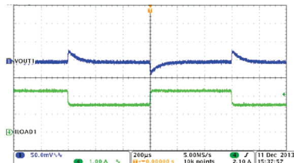
图 8-16. Buck1, Load Transient, 1.5 to 2.25 A SR = 0.25 A/μs
