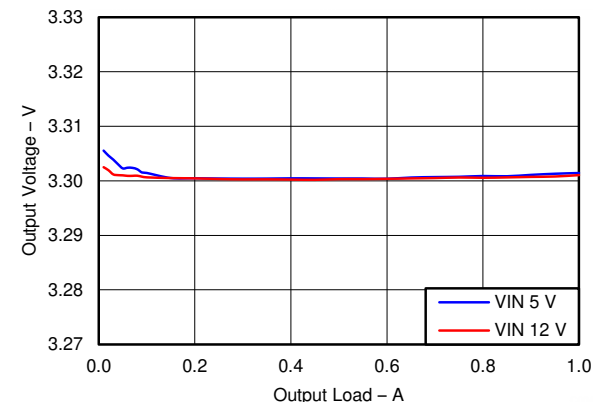
图 6-5. Buck3, Load Regulation
