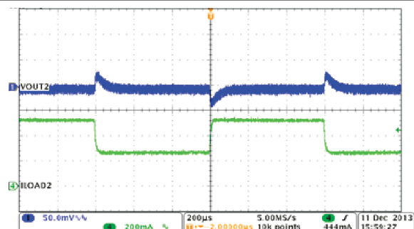
图 8-17. Buck2, Load Transient, 0.25 to 0.5 A SR = 0.25 A/μs
