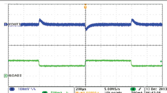
图 8-20. Buck3, Load Transient, 0.5 to 0.75 A SR = 0.25 A/μs
