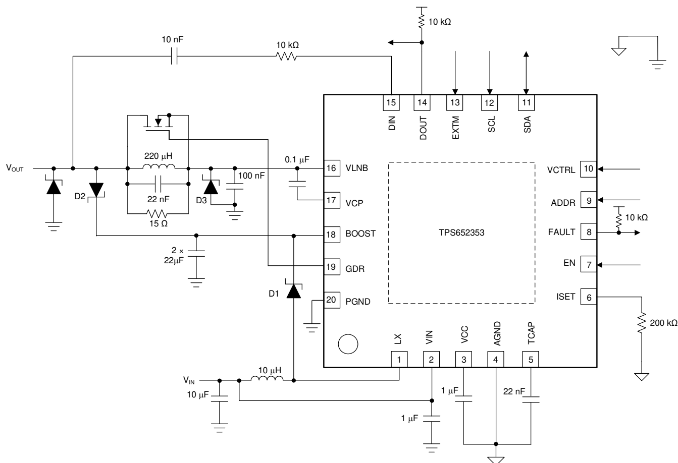
图 8-20. Application Schematic for DiSEq2.x Support
