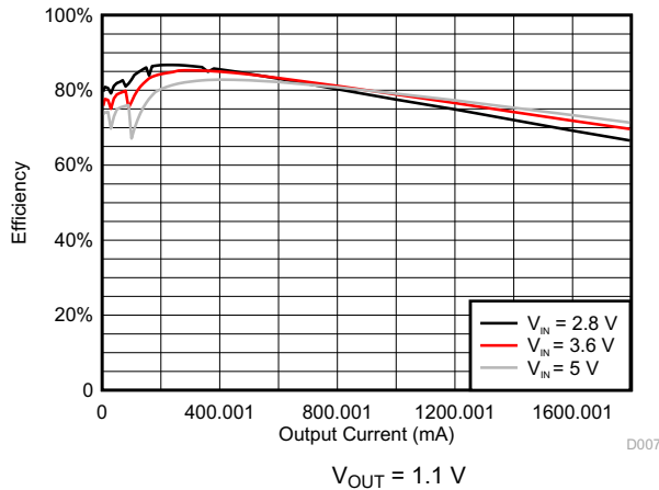
图 8-3. DCDC1/DCDC2 Efficiency
