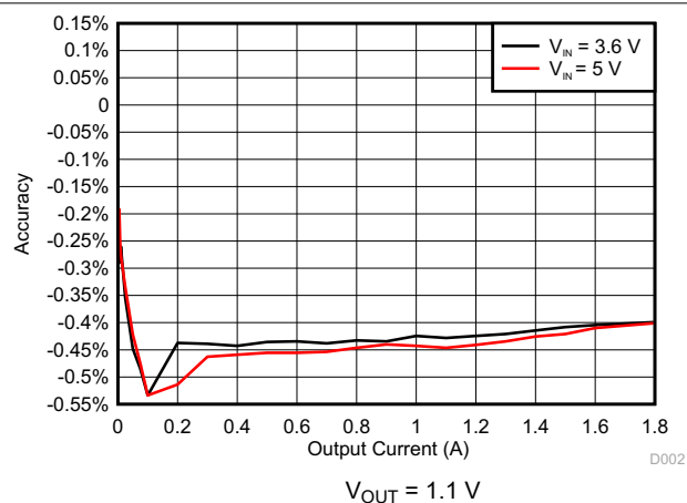
图 6-2. DCDC2 Accuracy
