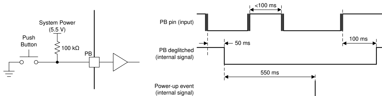
图 7-26. Left: Typical PB Input Circuit Right: Push-Button Input (PB) Deglitch and Power-Up Timing
