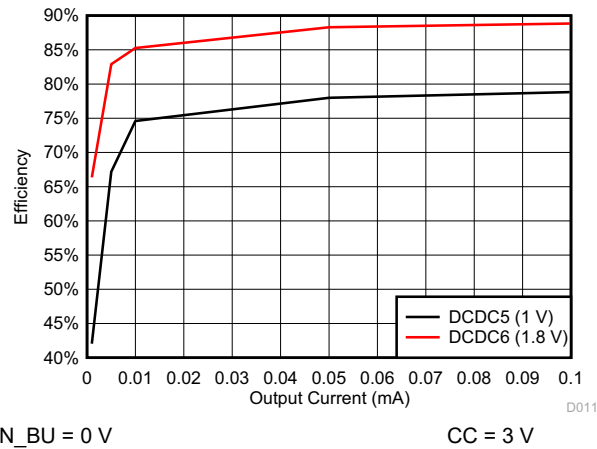
图 8-7. DCDC5/DCDC6 Efficiency
