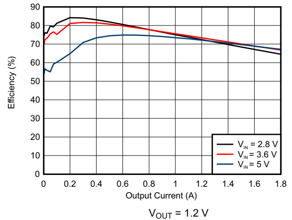
图 8-4. DCDC3 Efficiency
