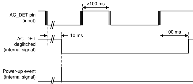
图 7-29. AC_DET Input Deglitch and Power-Up Timing (Portable Systems)
