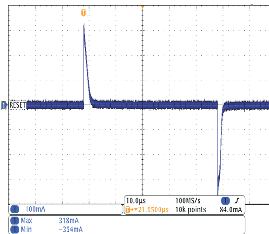
Figure 6-25. PEAK OUTPUT CURRENT - VST, RESET, etc.
