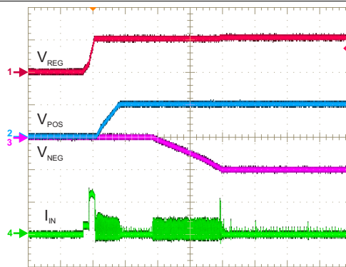
Figure 107. Inrush Current — Sequential SYNC = HIGH
