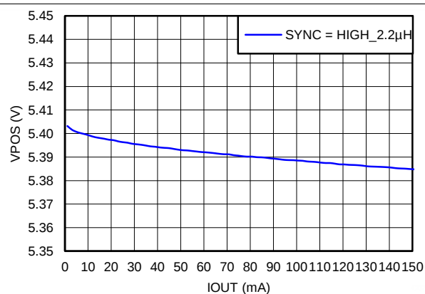
Figure 109. Load Regulation V_{POS} = 5.4\text{ V} — SYNC = HIGH
