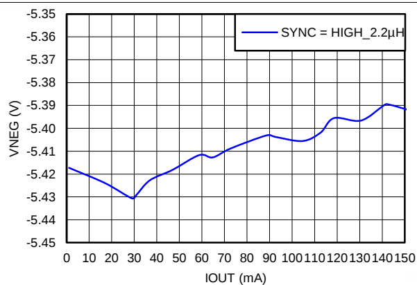
Figure 111. Load Regulation V_{NEG} = -5.4\text{ V} — SYNC = HIGH
