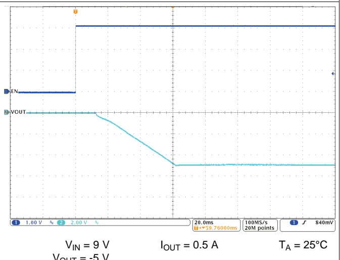
图 30. Start-Up Timing
