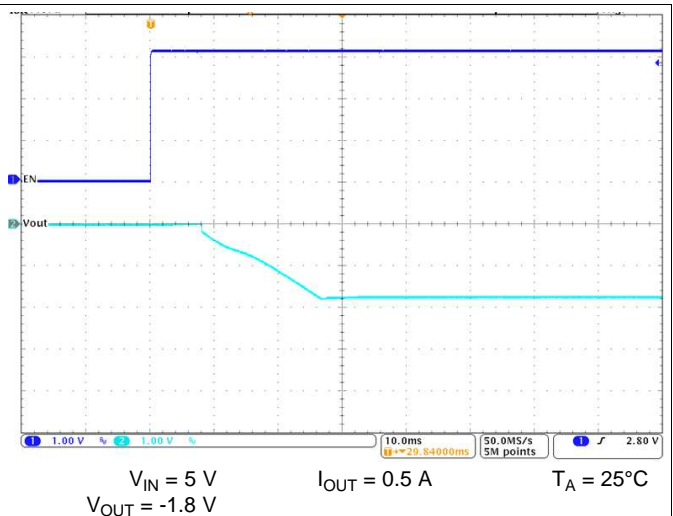
图 28. Start-Up Timing
