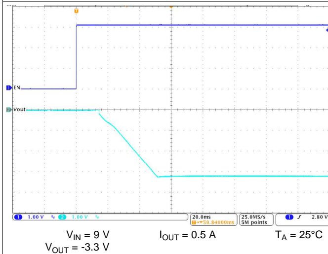
图 29. Start-Up Timing
