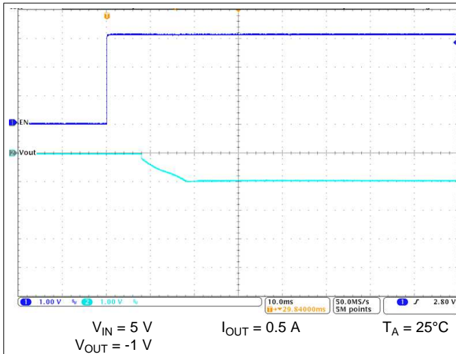
图 27. Start-Up Timing
