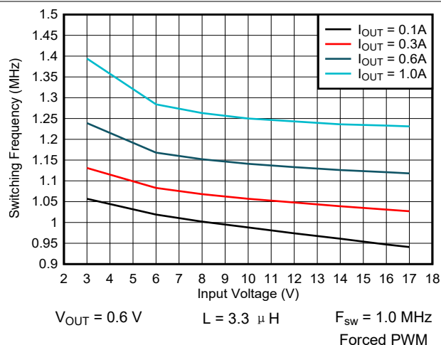
图 9-59. Switching Frequency vs Input Voltage
