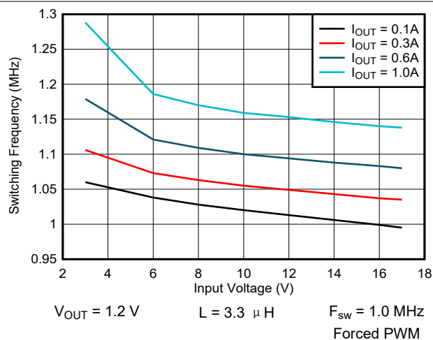
图 9-47. Switching Frequency vs Input Voltage
