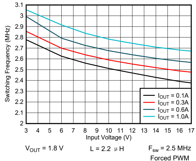
图 9-29. Switching Frequency vs Input Voltage
