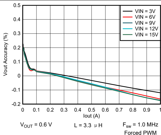
图 9-61. Output Voltage vs Output Current
