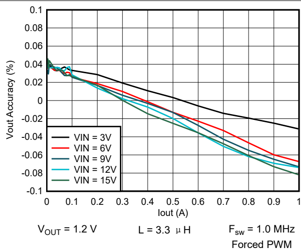
图 9-49. Output Voltage vs Output Current
