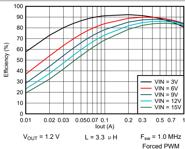
图 9-45. Efficiency vs Output Current
