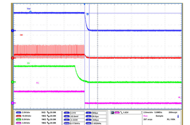
图 9-65. Shutdown Timing with Output Discharge Enabled
