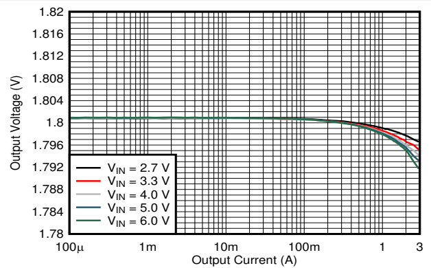
图 10-11. Output Voltage Versus Output Current
