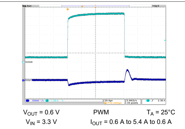
图 10-31. Load Transient Response
