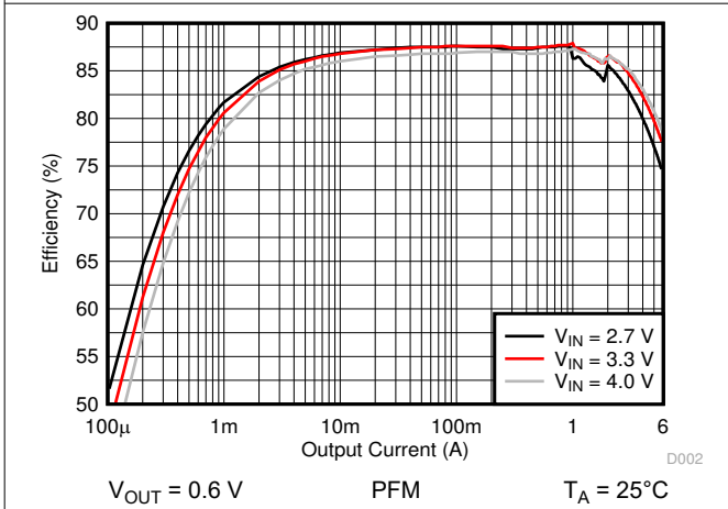
图 10-10. Efficiency Versus Output Current
