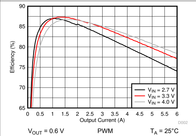
图 10-11. Efficiency Versus Output Current
