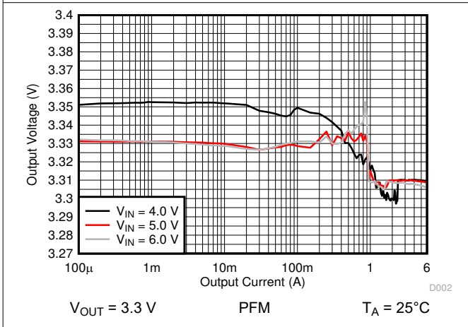
图 10-12. Output Voltage Versus Output Current
