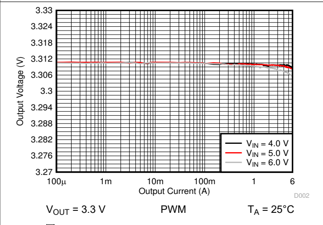
图 10-13. Output Voltage Versus Output Current
