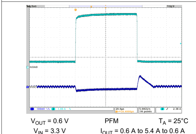
图 10-30. Load Transient Response
