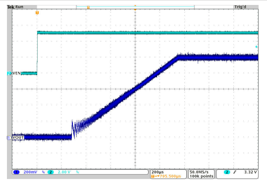
图 10-53. Start-Up Timing
