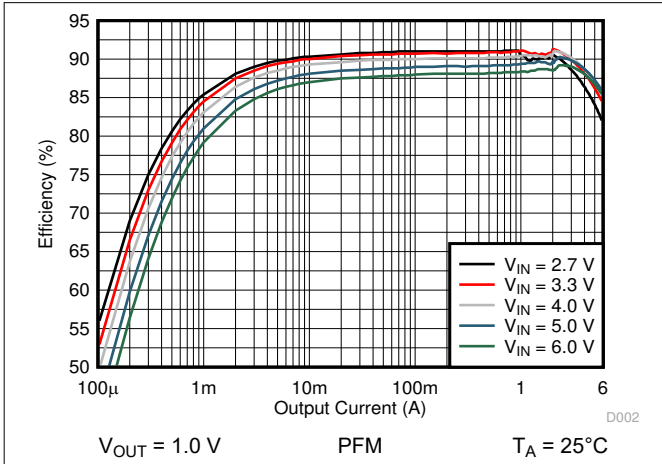
图 10-8. Efficiency Versus Output Current
