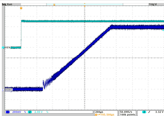
图 10-52. Start-Up Timing
