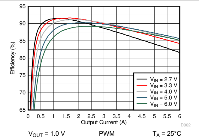
图 10-9. Efficiency Versus Output Current
