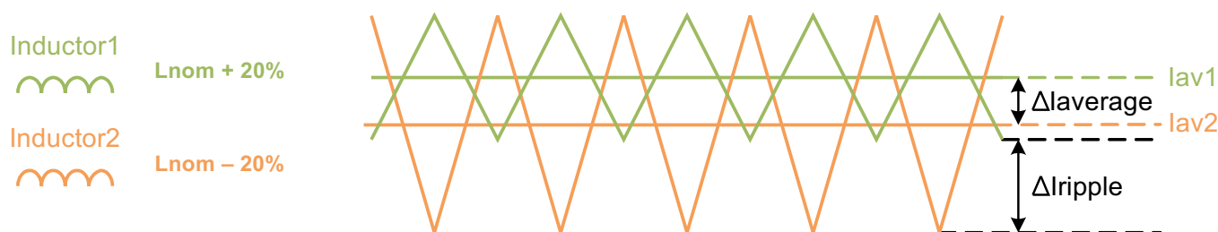
Figure 9. Inductor Currents
