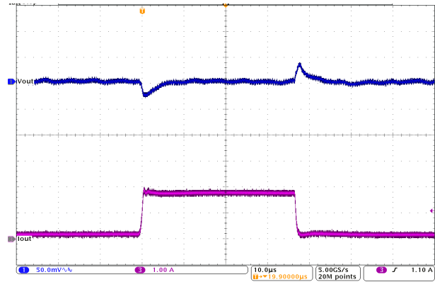
图 10-32. Load Transient Response
