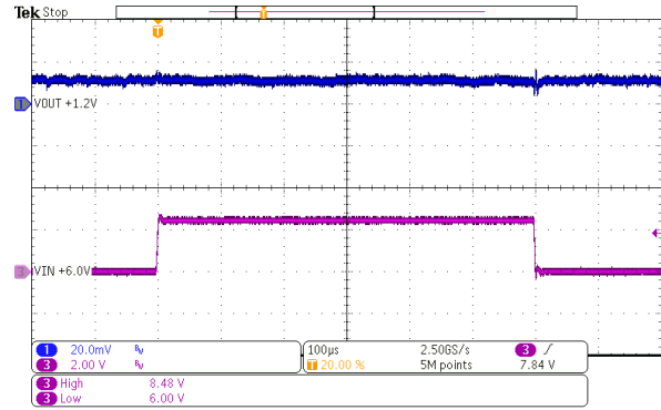
图 10-33. Line Transient Response
