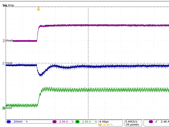
图 9-30. PWM-PSM-Transition
