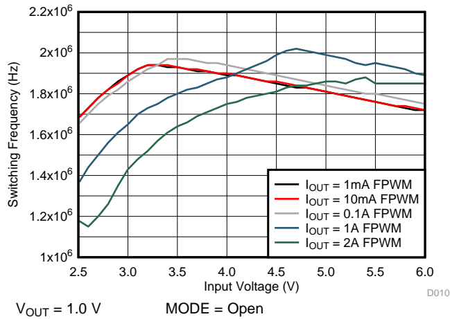
图 17. Switching Frequency, Forced PWM Mode (2.5MHz)
