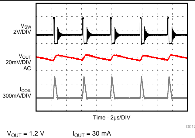
图 19. Output Ripple, PSM Operation
