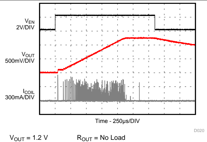
图 22. Startup and Shutdown without Load
