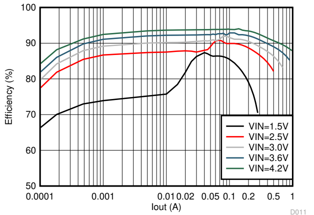
TPS613222A L = 2.2\text{ }\mu\text{H} D1:ZLLS410TA
