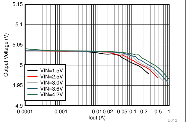
TPS613222A L = 2.2\text{ }\mu\text{H} D1:ZLLS410TA
