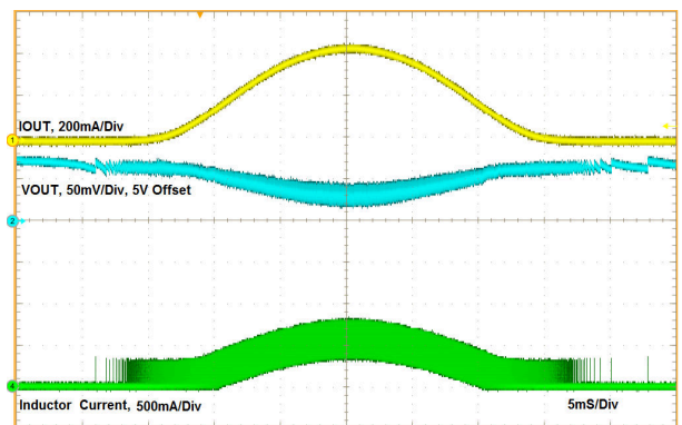
V_{IN} = 3.6\text{ V} TPS613222A I_{OUT} = 0\text{ mA to } 500\text{ mA}
