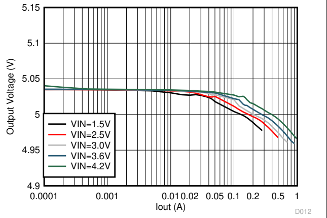
TPS613222A L = 2.2\text{ }\mu\text{H} D1:ZLLS410TA
