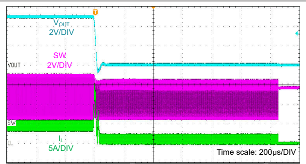
Figure 9-30. Output Short to Ground Protection
