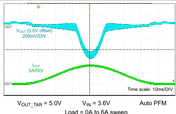
Figure 9-22. Load Sweep
