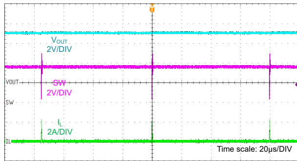
Figure 9-25. Current Limit Operation at Boost Mode
