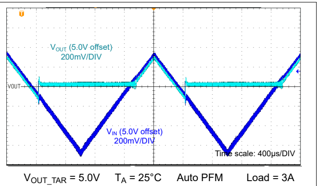
Figure 9-18. Boost to bypass Mode Exit / Entry
