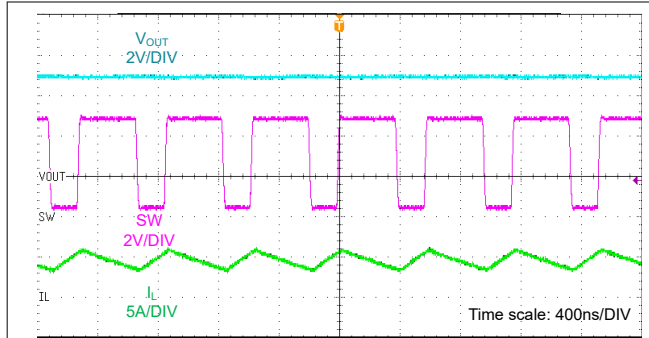
Figure 9-29. Switching Waveform at Heavy Load
