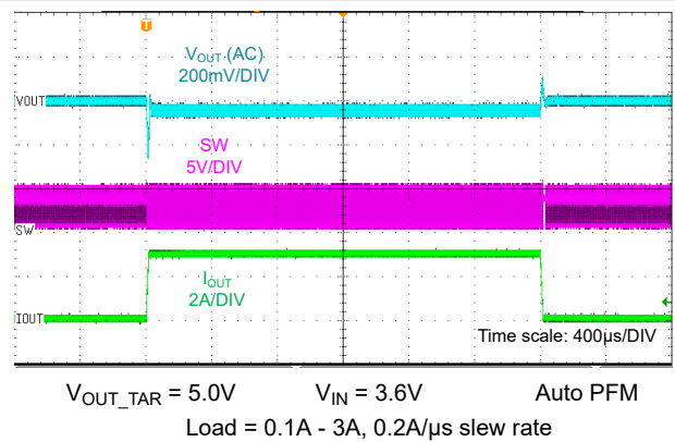
Figure 9-20. Load Transient Response
