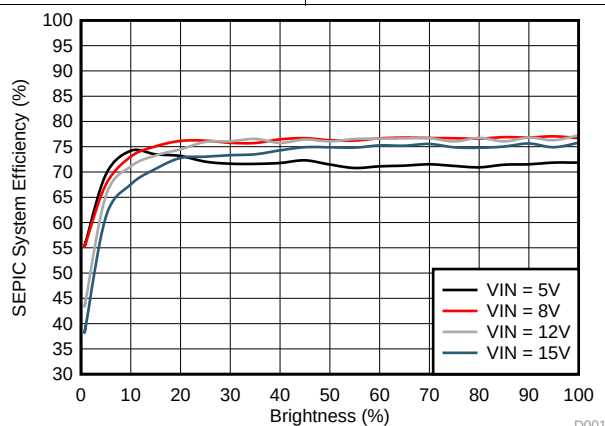
Figure 26. SEPIC Efficiency
