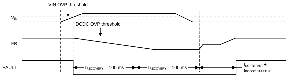
Figure 14. V_{\text{IN}} Overvoltage Protection ( V_{\text{IN}} OVP)
