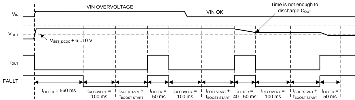
Figure 13. V_{\text{IN}} Overvoltage Protection (DC-DC OVP)
