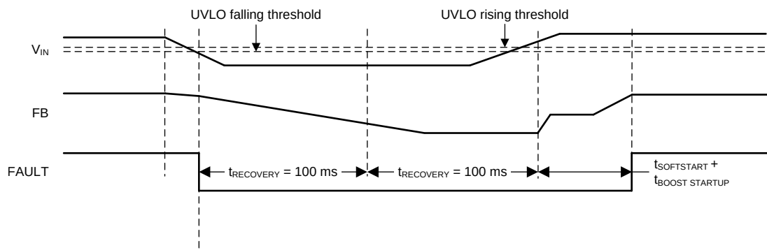
Figure 15. V_{\text{IN}} Undervoltage Lockout
