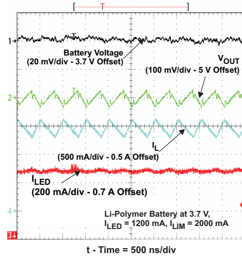
Figure 46. Input Ripple Voltage
