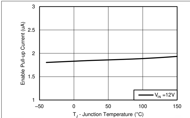
图 6-7. Enable Pull-Up Current, V_{EN} = 1.0V
