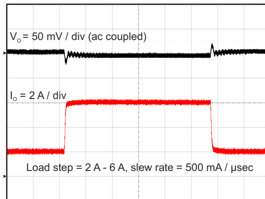
图 8-18. Transient Response
