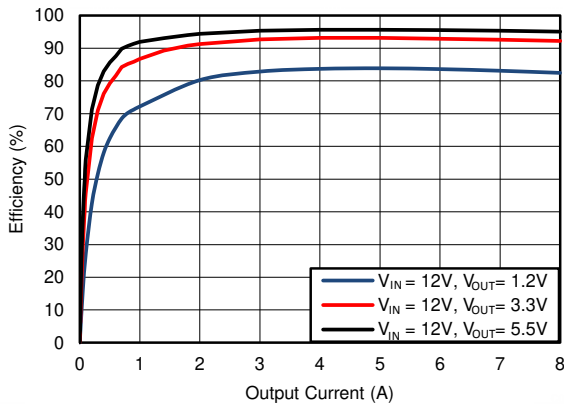
图 6-15. Efficiency, Mode = FFCM, F_{SW} = 1200\text{kHz}
