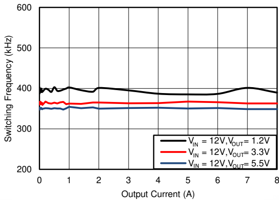
图 6-17. F_{SW} Load Regulation, Mode = FFCM, F_{SW} = 400\text{kHz}
