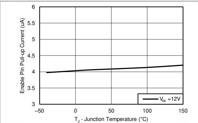
图 6-8. Enable Pull-Up Current, V_{EN} = 1.3V
