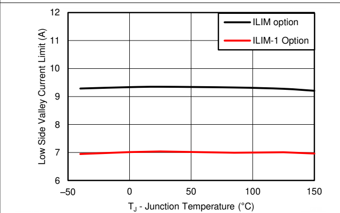
图 6-10. Valley Current Limit vs Temperature
