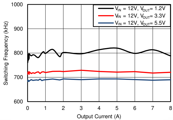
图 6-18. F_{SW} Load Regulation, Mode = FFCM, F_{SW} = 800\text{kHz}
