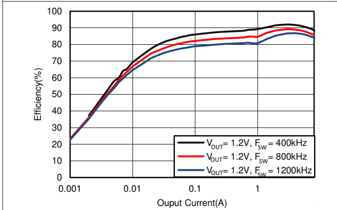
图 6-11. Efficiency with Internal VREG5 = 4.7 V, V_{IN} = 12 V
