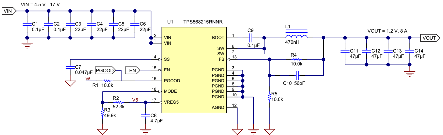
图 8-1. Application Schematic
