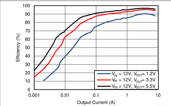
图 6-12. Efficiency, Mode = DCM, F_{SW} = 400kHz
