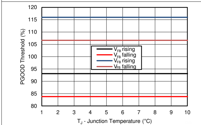
图 6-9. PGOOD Threshold vs Temperature
