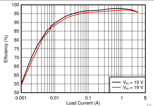
图 12. V_{OUT}=3.3\text{ V} Efficiency, L=4.7\text{ }\mu\text{H}
