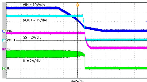
图 8-9. Shutdown Relative to V_{IN} , I_{OUT} = 3\text{ A}
