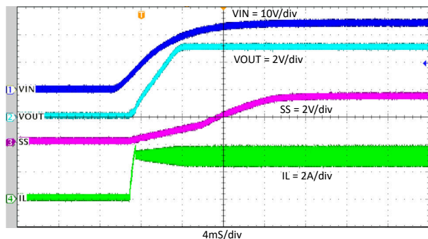
图 8-8. Start-Up Relative to V_{IN} , I_{OUT} = 3\text{ A}
