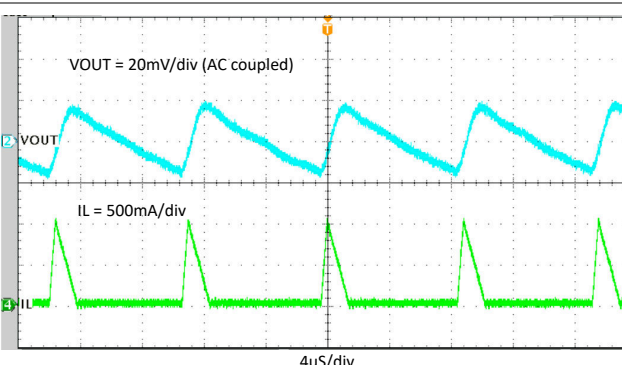
图 8-13. Steady State, I_{OUT} = 0.1\text{ A}
