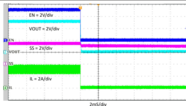
图 8-11. Shutdown Through EN, I_{OUT} = 3\text{ A}
