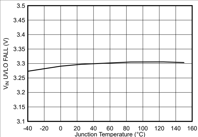
图 6-8. V IN UVLO Falling Threshold vs Junction Temperature
